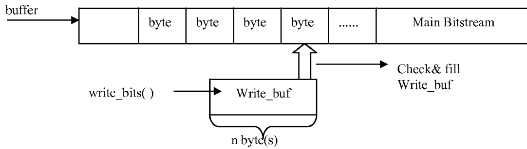
Encoder Bitstream
