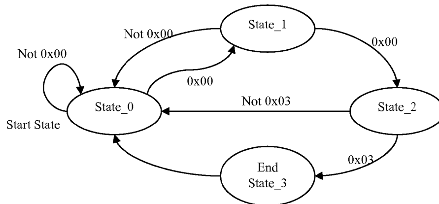
Decoder State Machine
