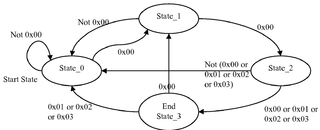
Encoder State Machine
