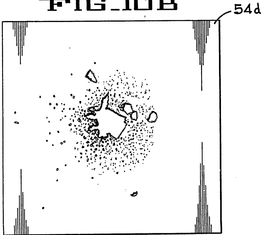
FRONT OF WITNESS WITNESS FROM SHOT NO. 46 WARHEAD: TOW II AT 0° TARGET: 1" 7039/.38" ALP
