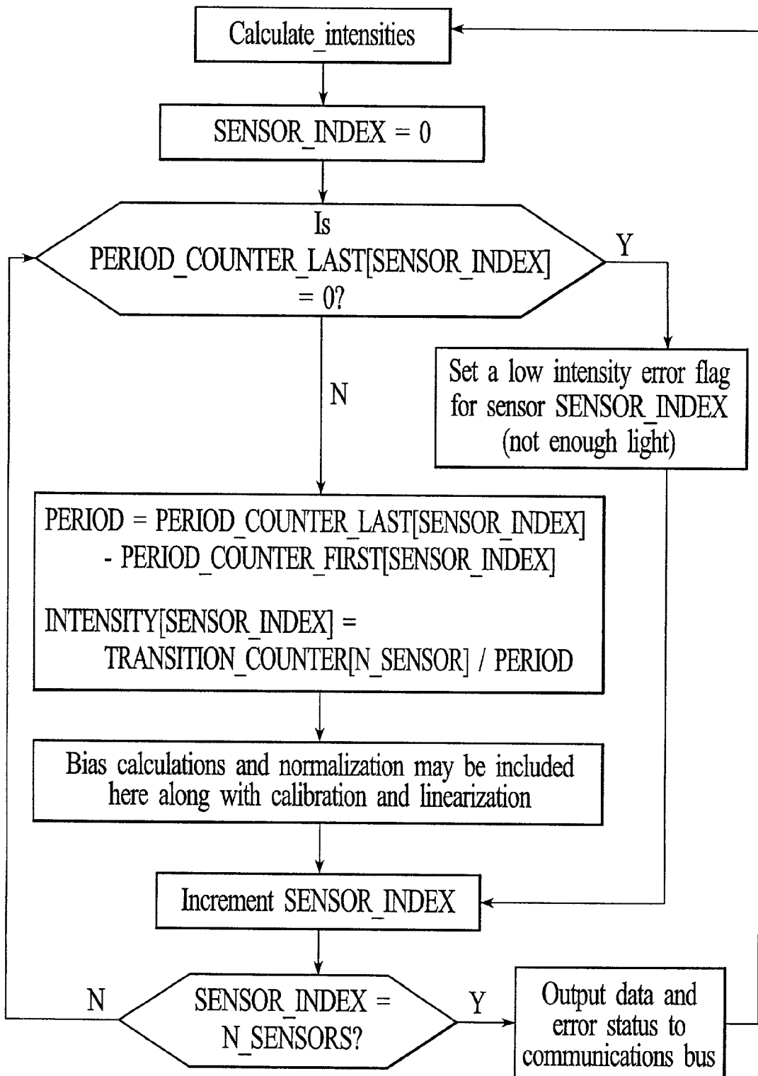
Intensity Calculations Flow Chart FIG. 90E
