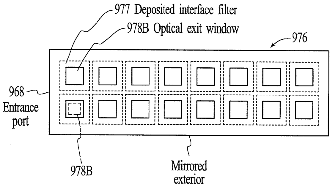
Optical Manifold FIG. 74A
