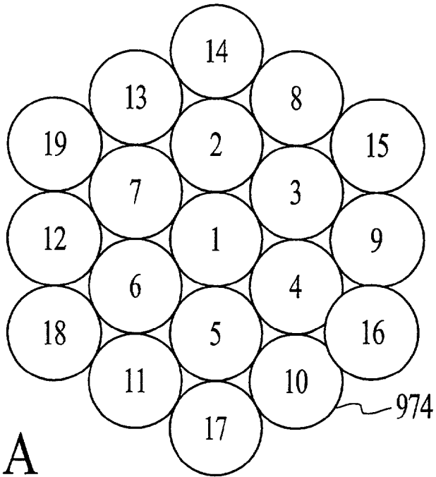
Non-Coherent Light Guide End View A
