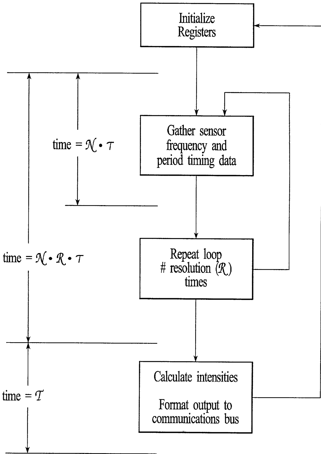
RISC Software Timing Flow Chart FIG. 90A
