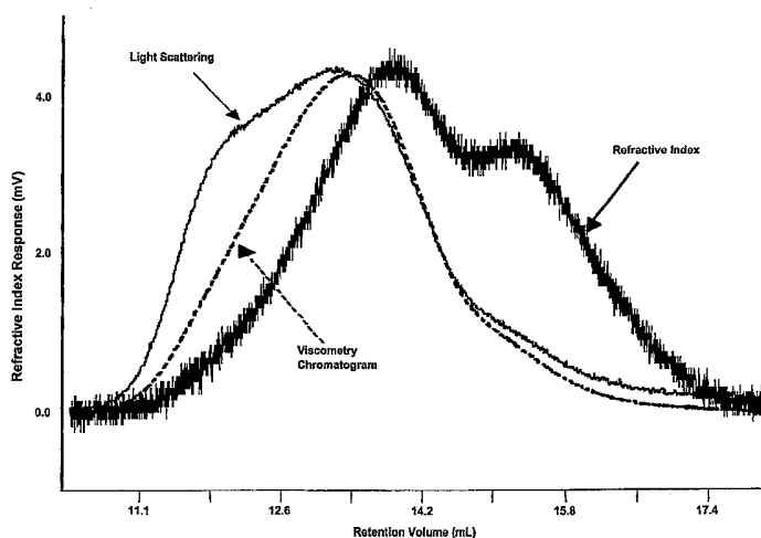
Typical chromatograms of CMC using aqueous SEC with triple detection (Neat CMC-MV)
