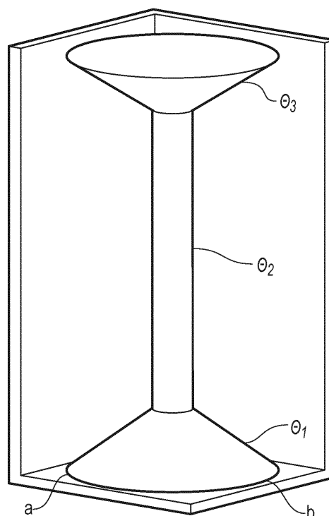
A Open view of hourglass resonator
