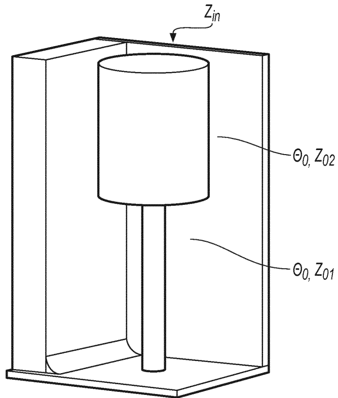
Stepped impedance resonator
