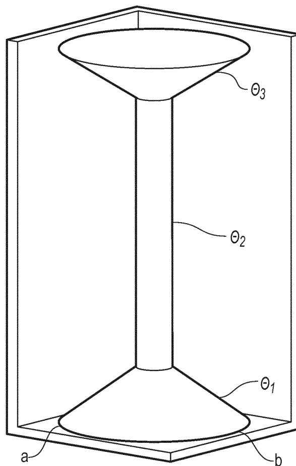
A Open view of hourglass resonator
