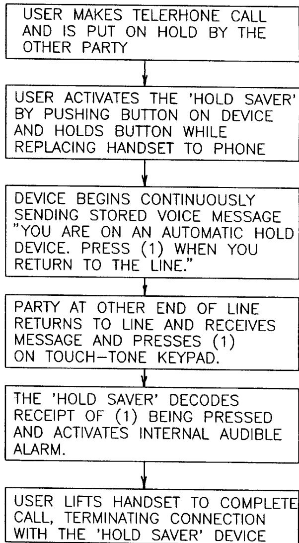
FIG 5 SEQUENCE OF OPERATION
