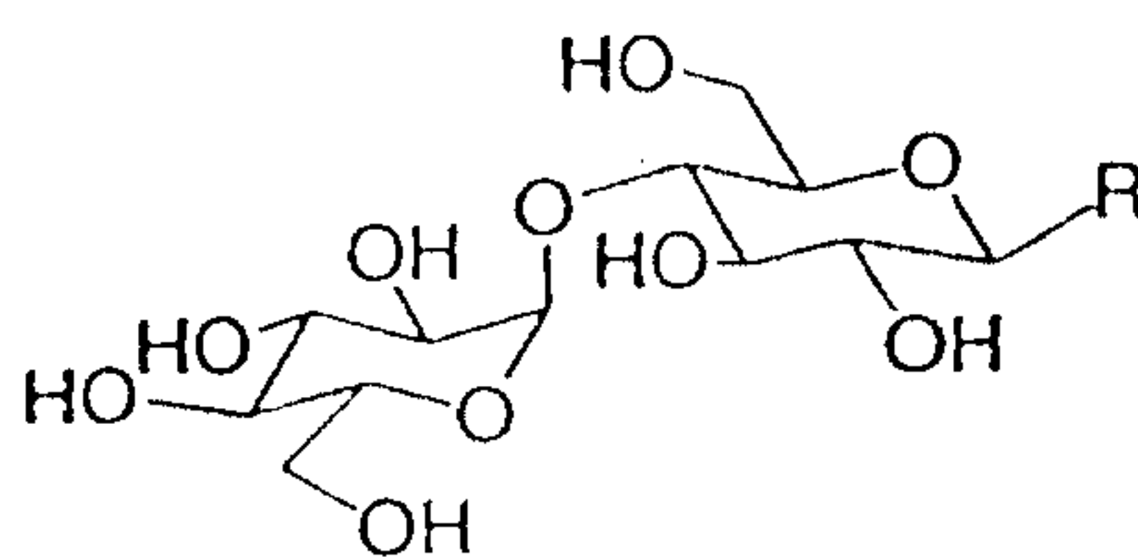
4. Maltose
