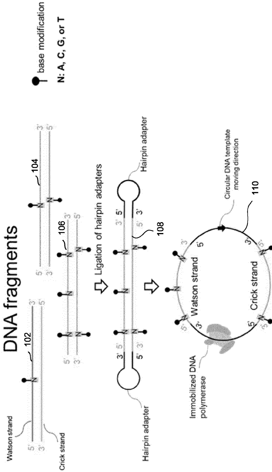
Single molecule real-time (SMRT) circular consensus sequencing
