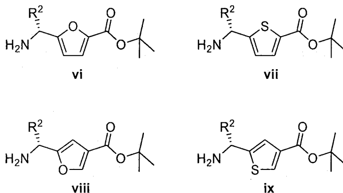
Figure 1: Examples of enantiomerically pure amines accessible via route outlined in Scheme 1
