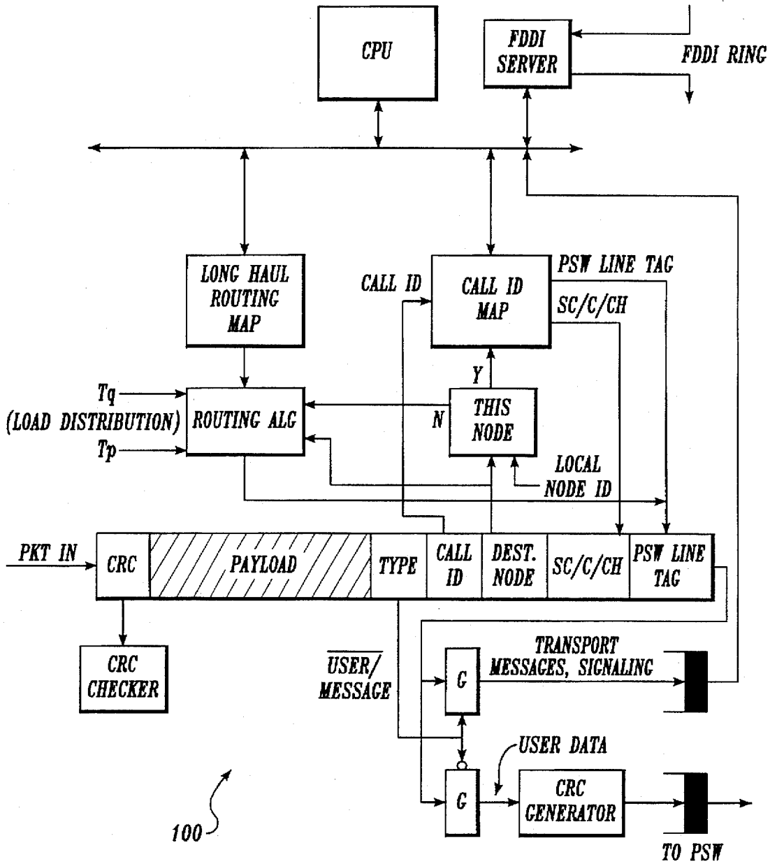
IPP: INPUT PACKET PROCESSOR
