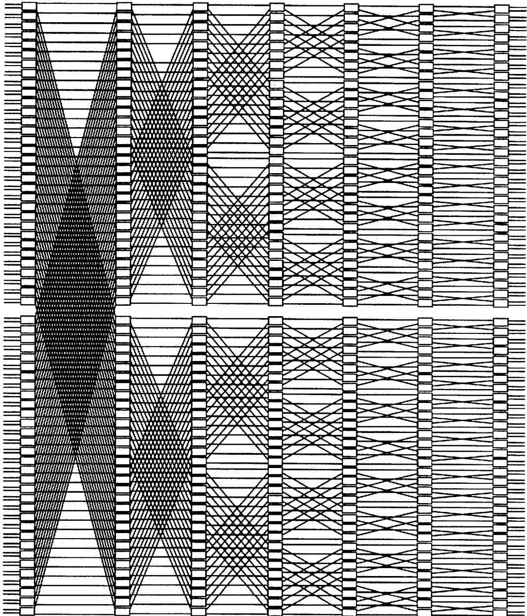
128X128 SWITCH
