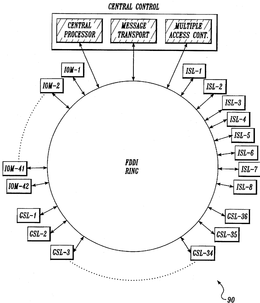
DISTRIBUTED CONTROL ARCHITECTURE
