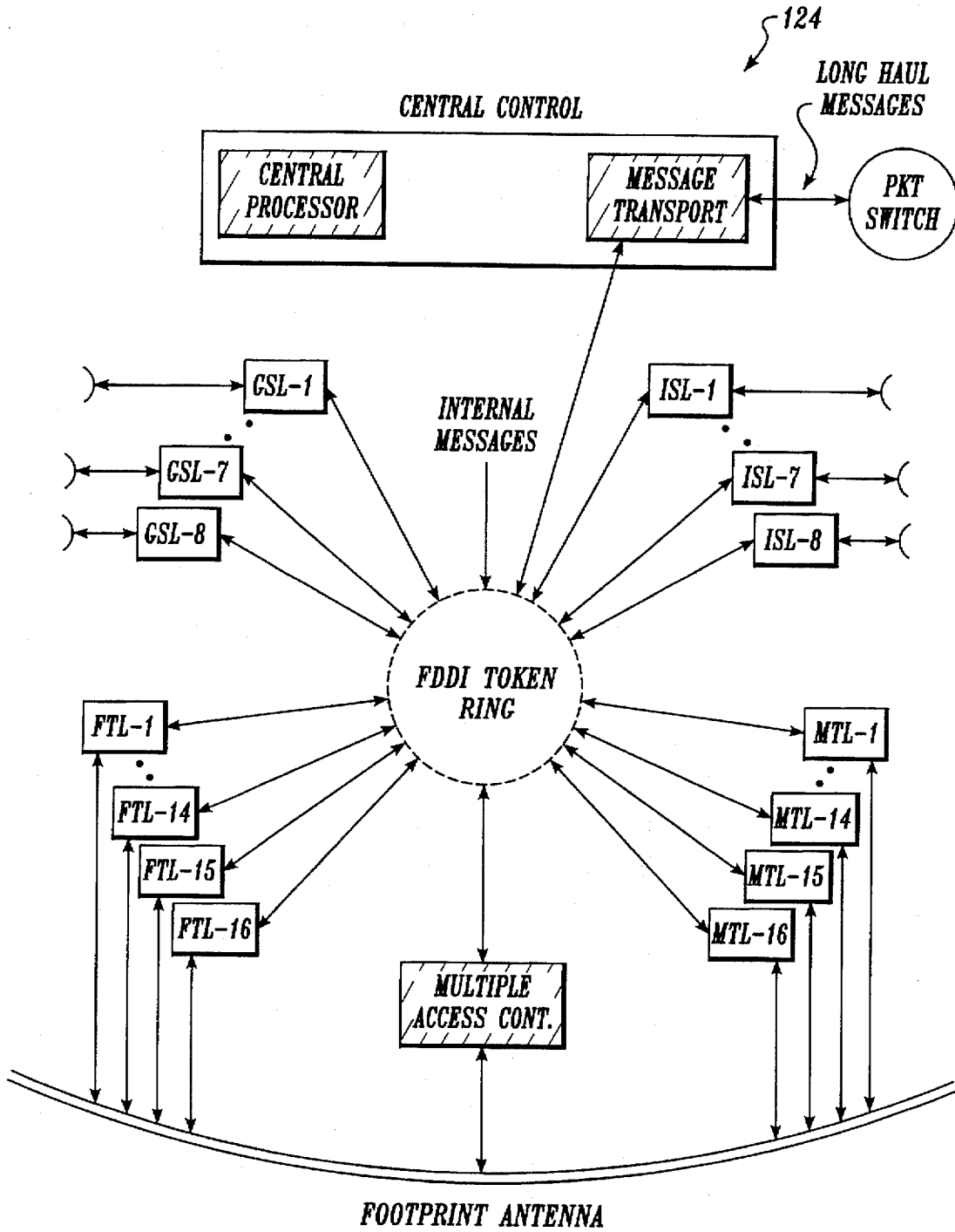
SYSTEM MESSAGE SWITCHING ARCHITECTURE
