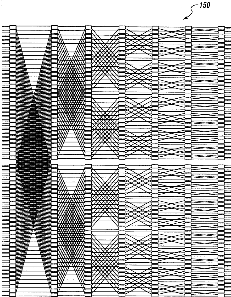
128X128 SWITCH
