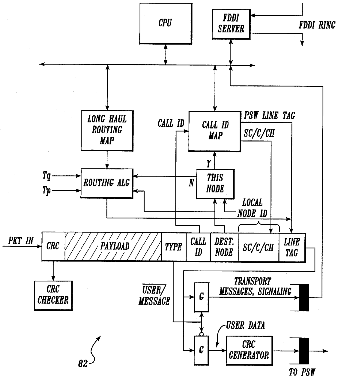
PACKET ROUTER
