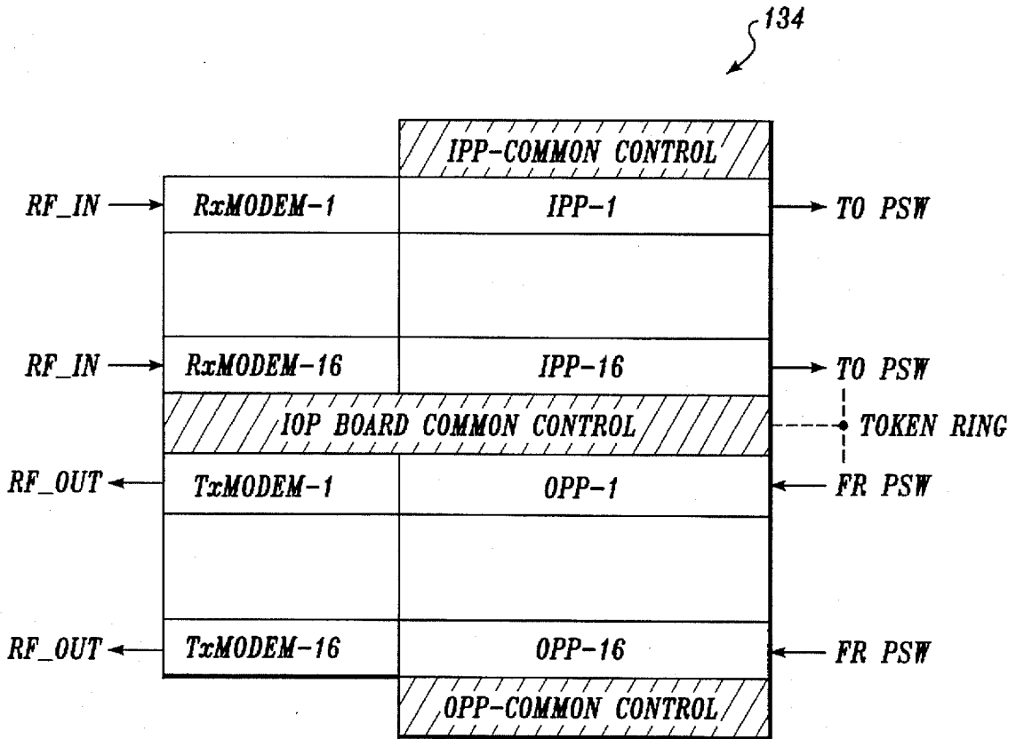
INPUT OUTPUT PACKET PROCESSOR BOARD
