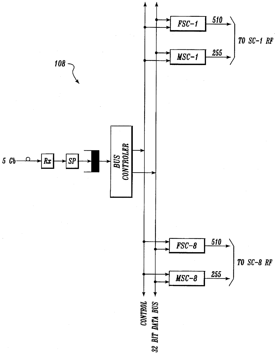
OM: FOOTPRINT OUTPUT MODULE (1/42)
