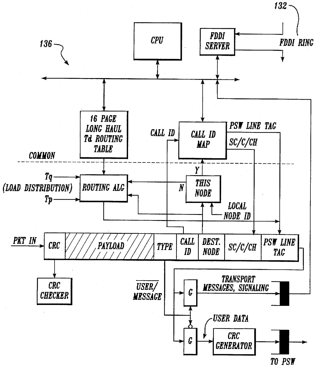
IPP: INPUT PACKET PROCESSOR
