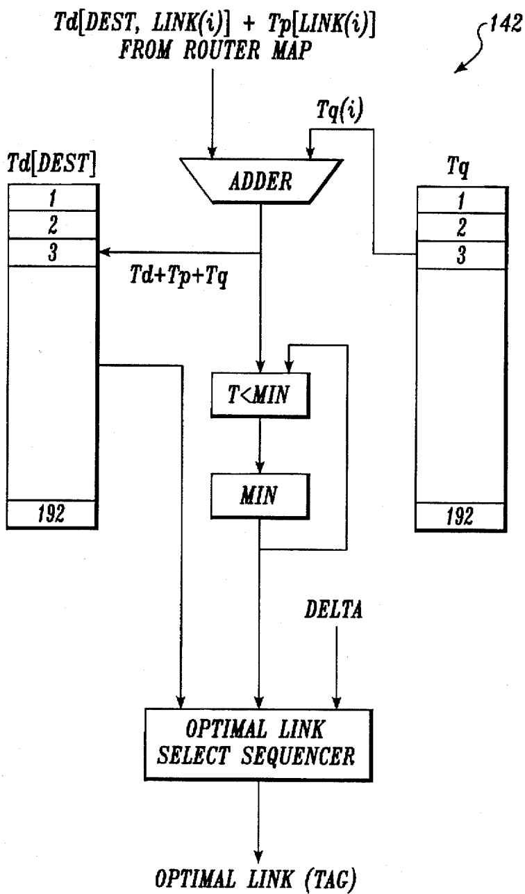
IPP OPTIMAL ROUTE CONTROLLER
