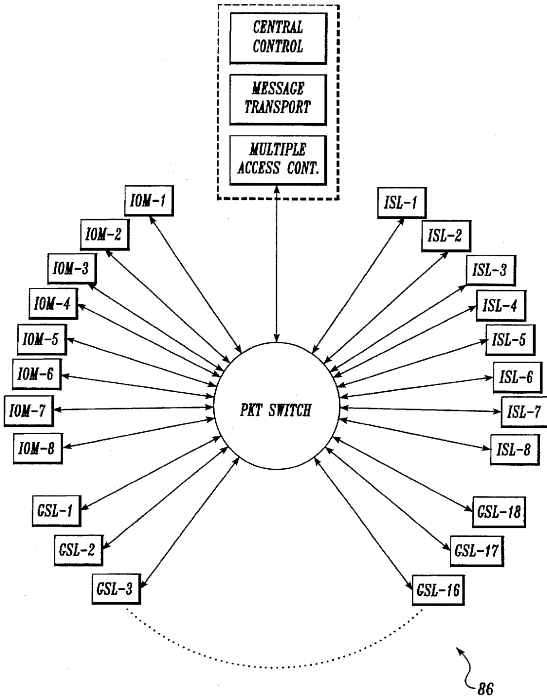
SYSTEM ARCHITECTURE
