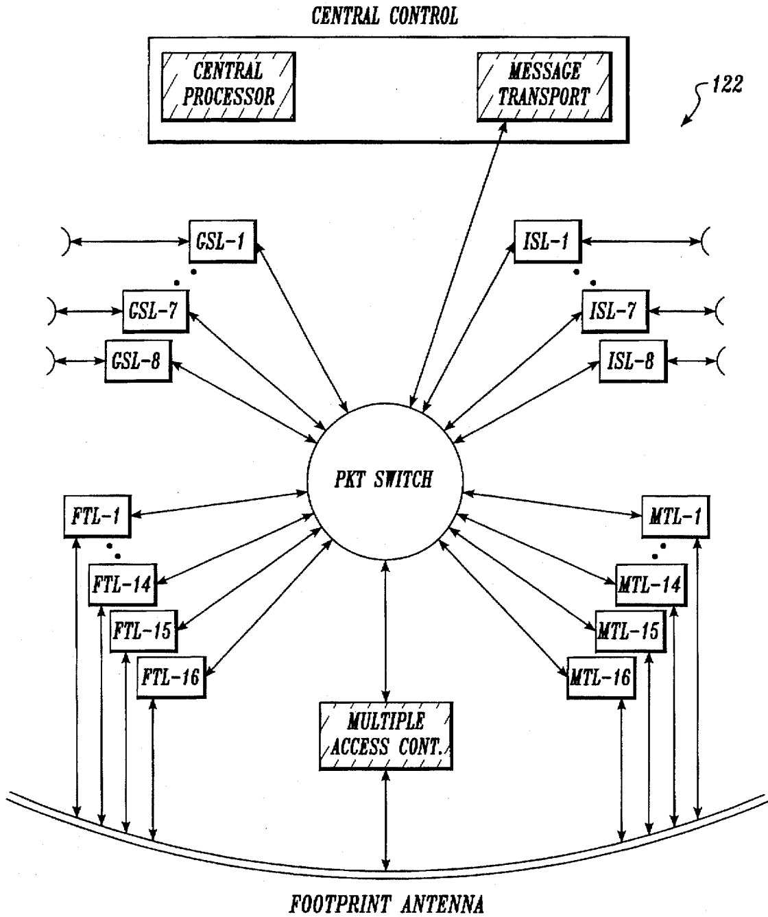
SYSTEM ARCHITECTURE
