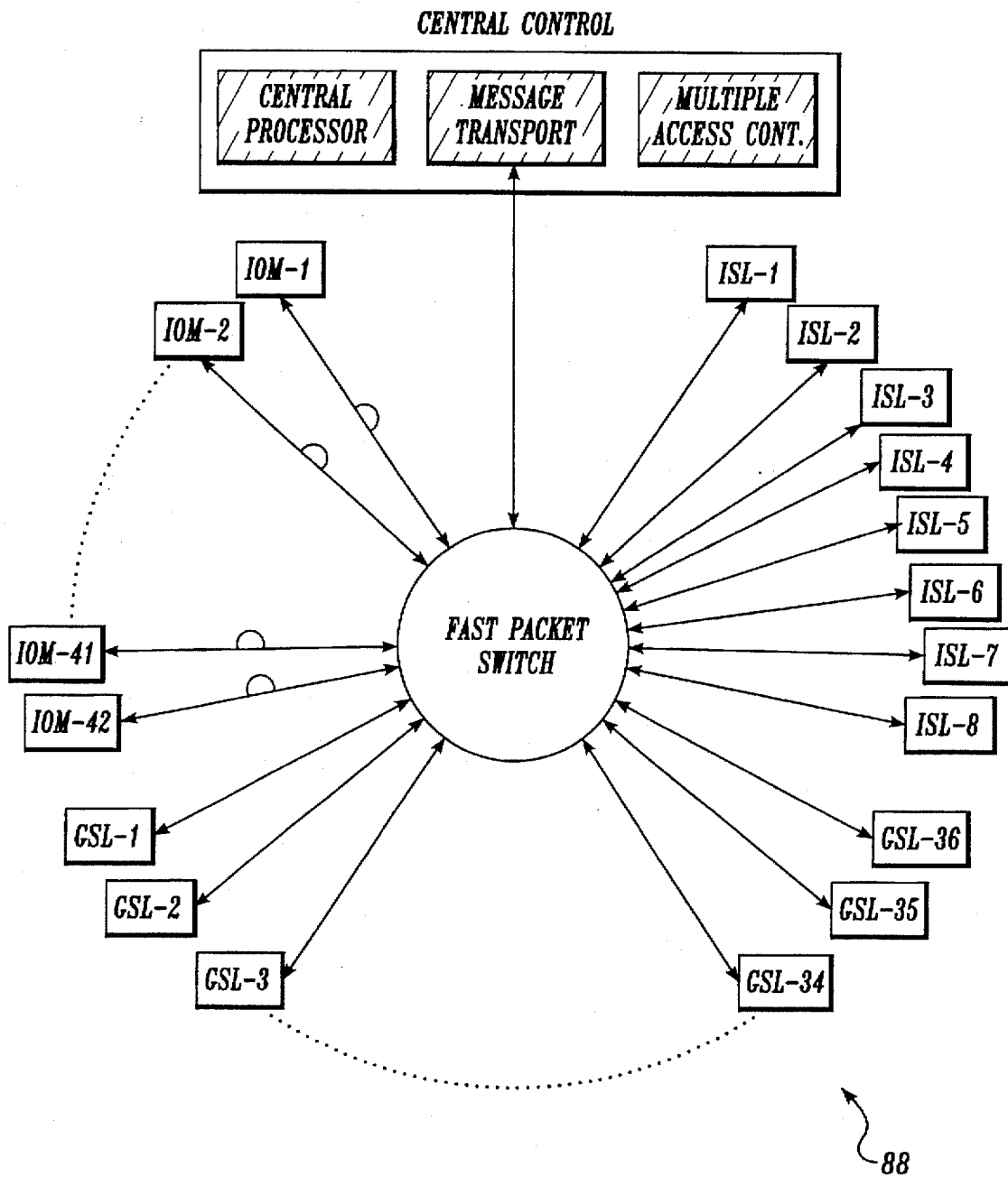
SWITCH ARCHITECTURE
