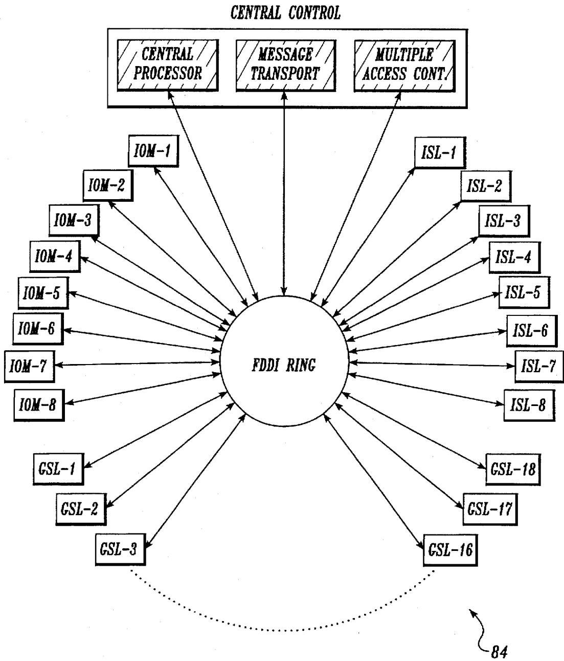
SYSTEM MESSAGE SWITCHING ARCHITECTURE
