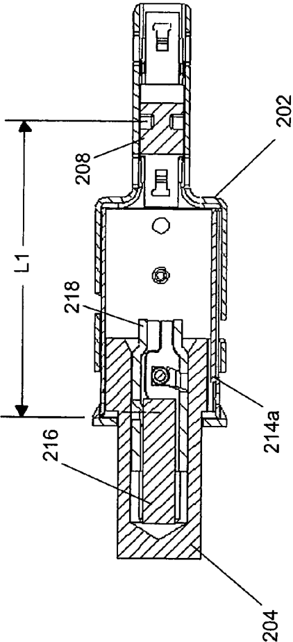
SECTION H-H
