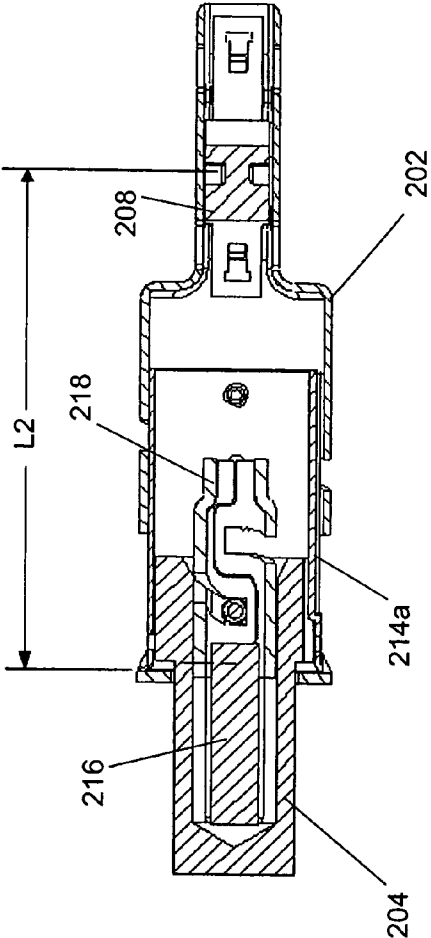
SECTION H'-H'
