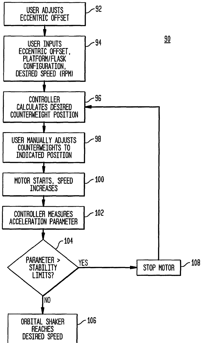
FIG. 9 MANUAL ADJUSTMENT
