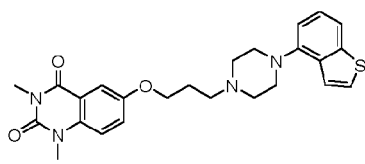
Compound D
