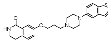
Compound C
