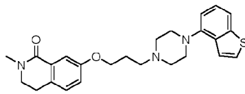
Compound B
