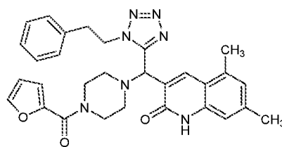
dimethylquinolin-2(1H)-one (GT996)
