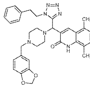
5,8-dimethylquinolin-2(1H)-one (GT867)
