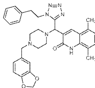
methyl-5,8-dimethylquinolin-2(1H)-one (GT867)
