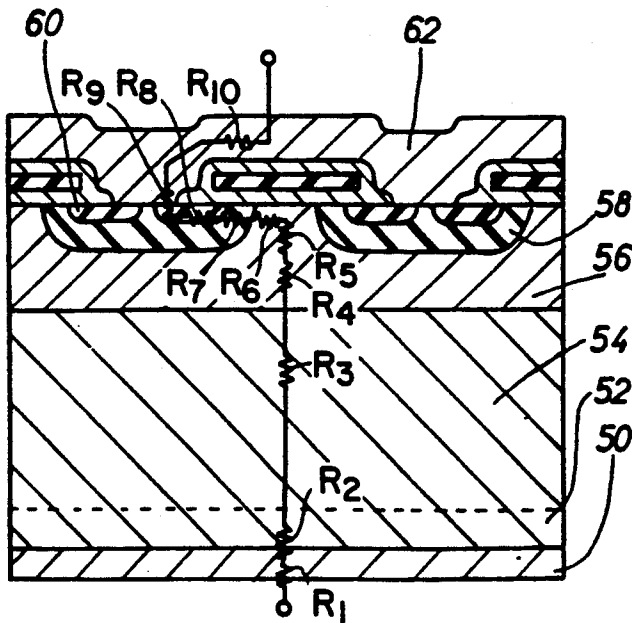
FIG. 13 (PRIOR ART)
