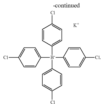
Potassium tetrakis(4-chlorophenyl)borate
