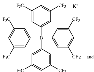
Potassium tetrakis[3,5-bis(trifluoromethyl)phenyl]borate or Sodium tetrakis[3,5-bis(trifluoromethyl)phenyl]borate
