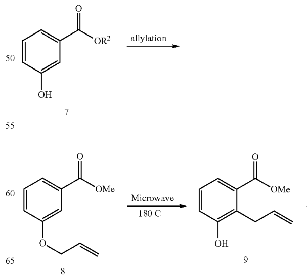
Scheme-2: Claisen Route to UT-15
