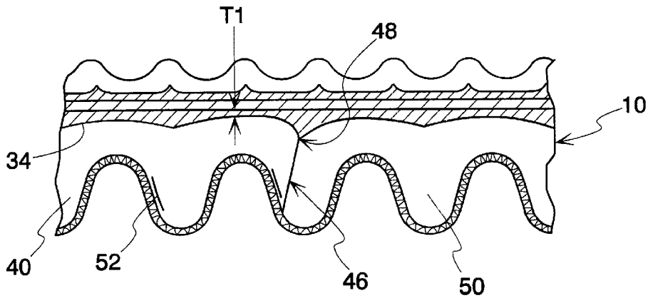
Fig. 9 (PRIOR ART)
