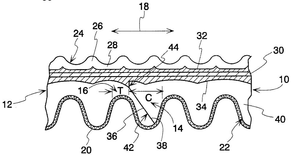
Fig. 8 (PRIOR ART)
