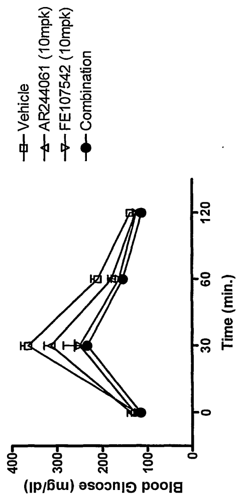
Figure 9A. GPR119 Agonist AR244061 and FE107542 Combination-1
