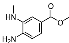
Intermediate 16
