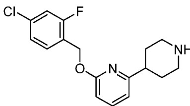
Intermediate 3
