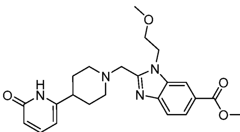
Intermediate 35
