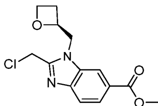
Intermediate 23
