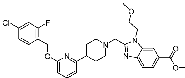
Intermediate 34
