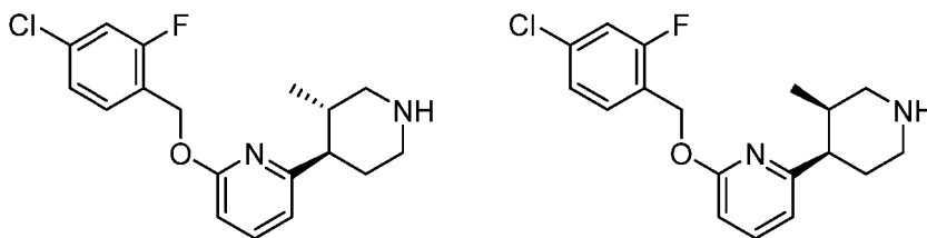
Intermediate 12a
