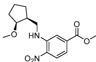
Intermediate 28
