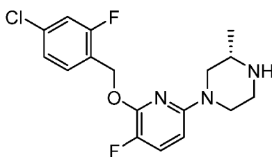
Intermediate 14
