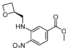
Intermediate 21
