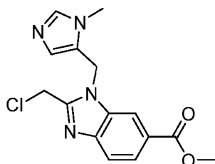
Intermediate 32
