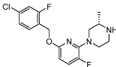
Intermediate 15
