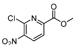
Intermediate 24
