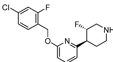
Intermediate 10
