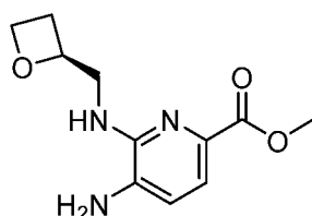
Intermediate 26
