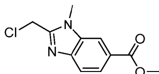
Intermediate 17
