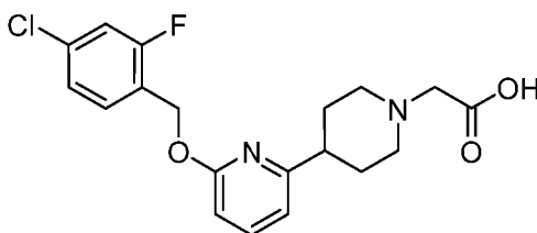
Intermediate 5
