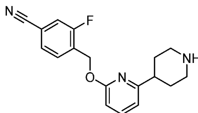
Intermediate 4
