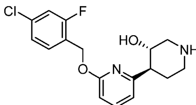
Intermediate 9
