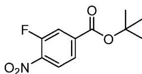
Intermediate 29
