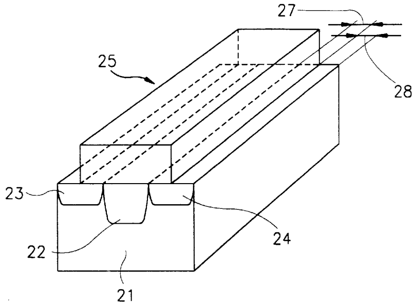
FIG. 2B CONVENTIONAL ART
