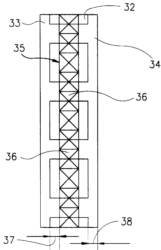
FIG. 3B CONVENTIONAL ART
