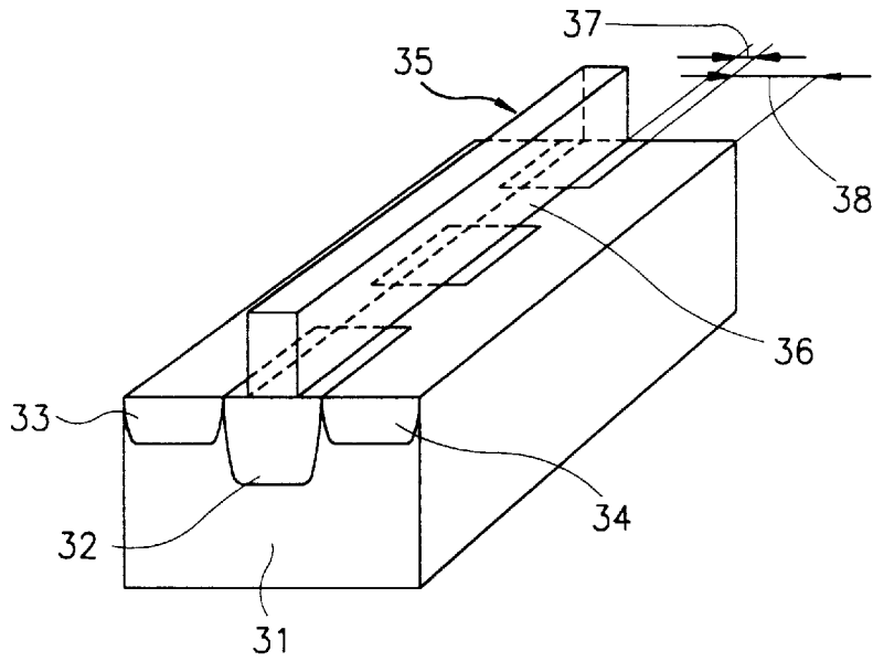
FIG. 3A CONVENTIONAL ART
