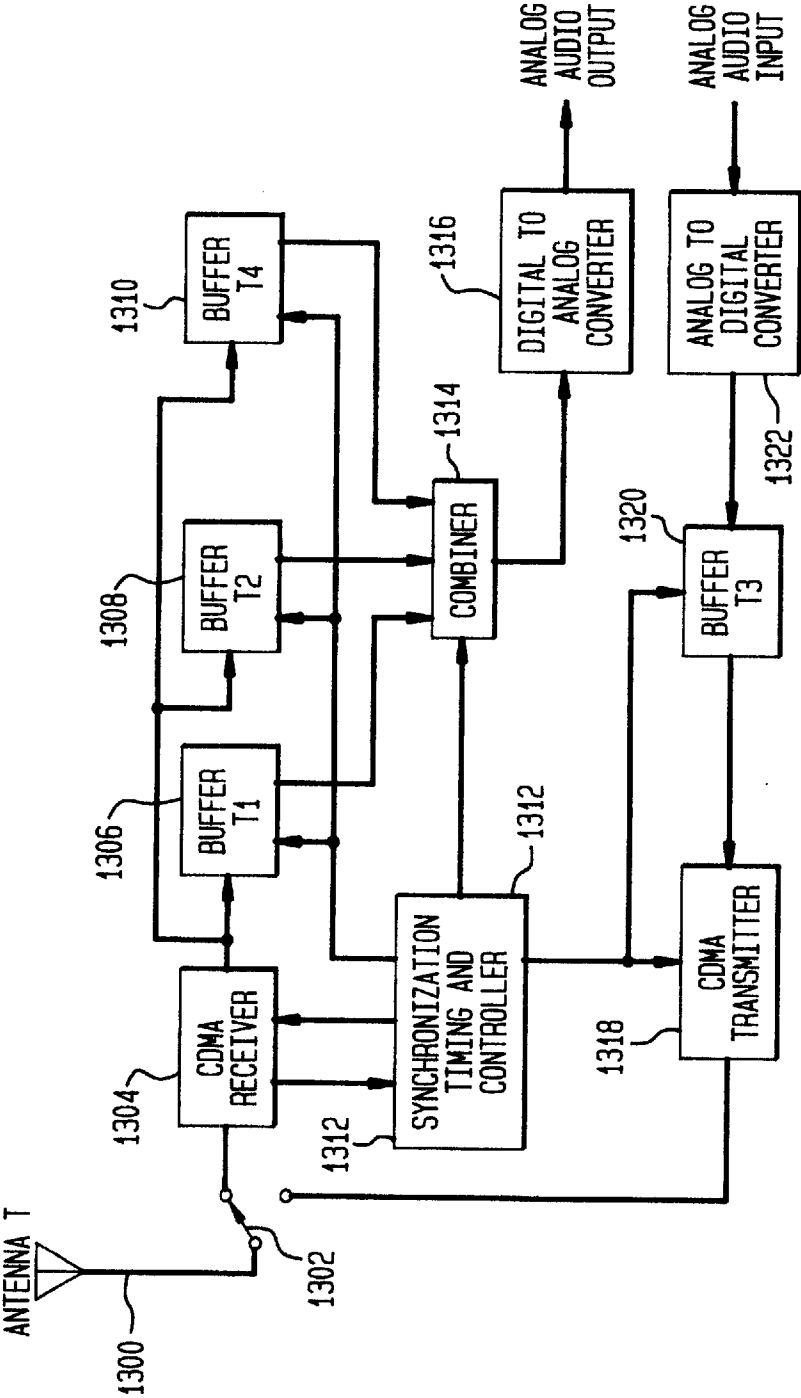
FIG. 13 SUBSCRIBER STATION
