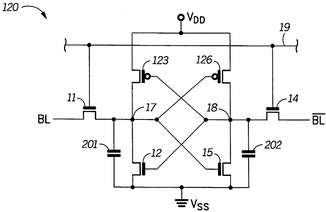
FIG. 12 -PRIOR ART-
