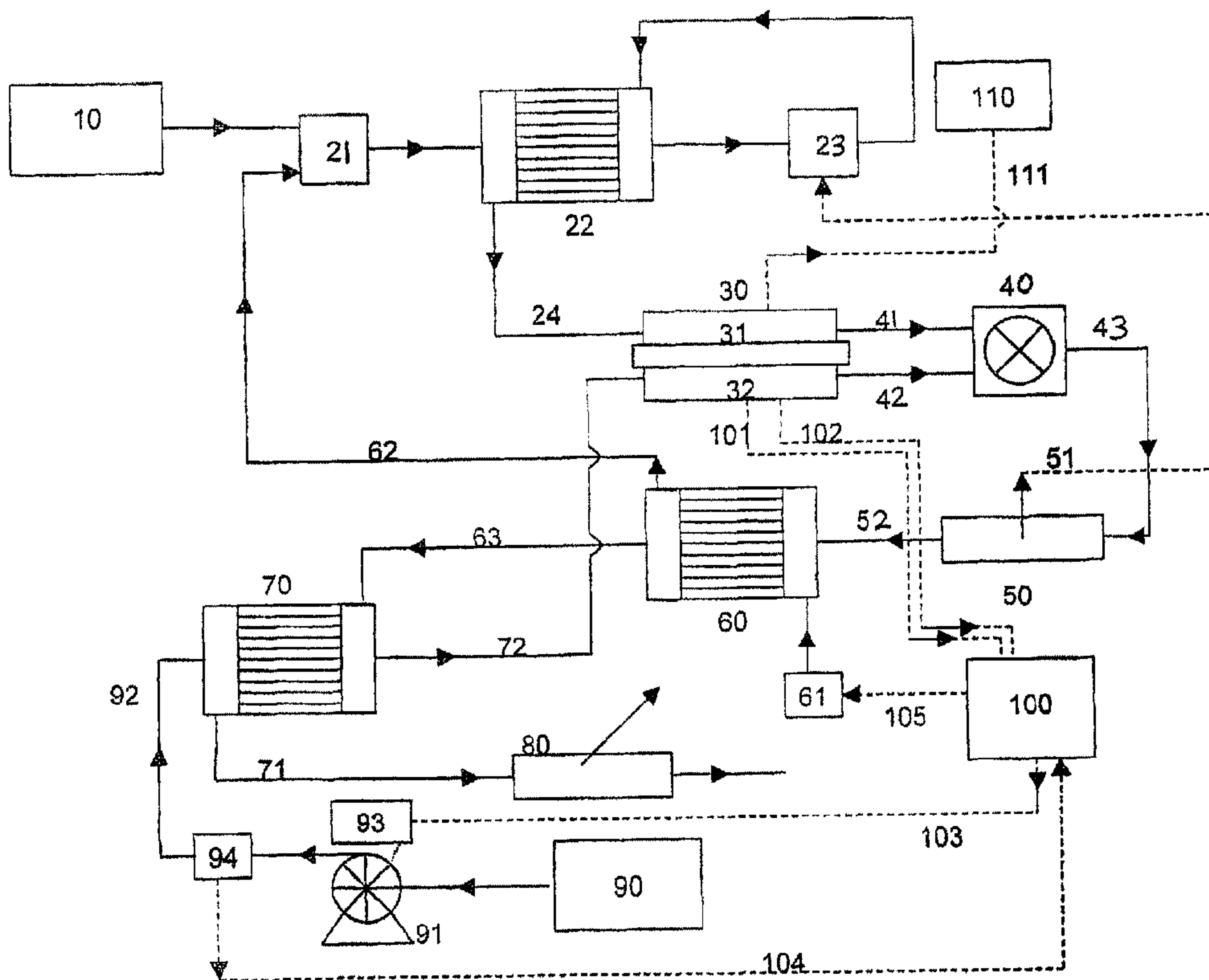
SOFC system operating on LPG showing method of implementation described in Method 1
