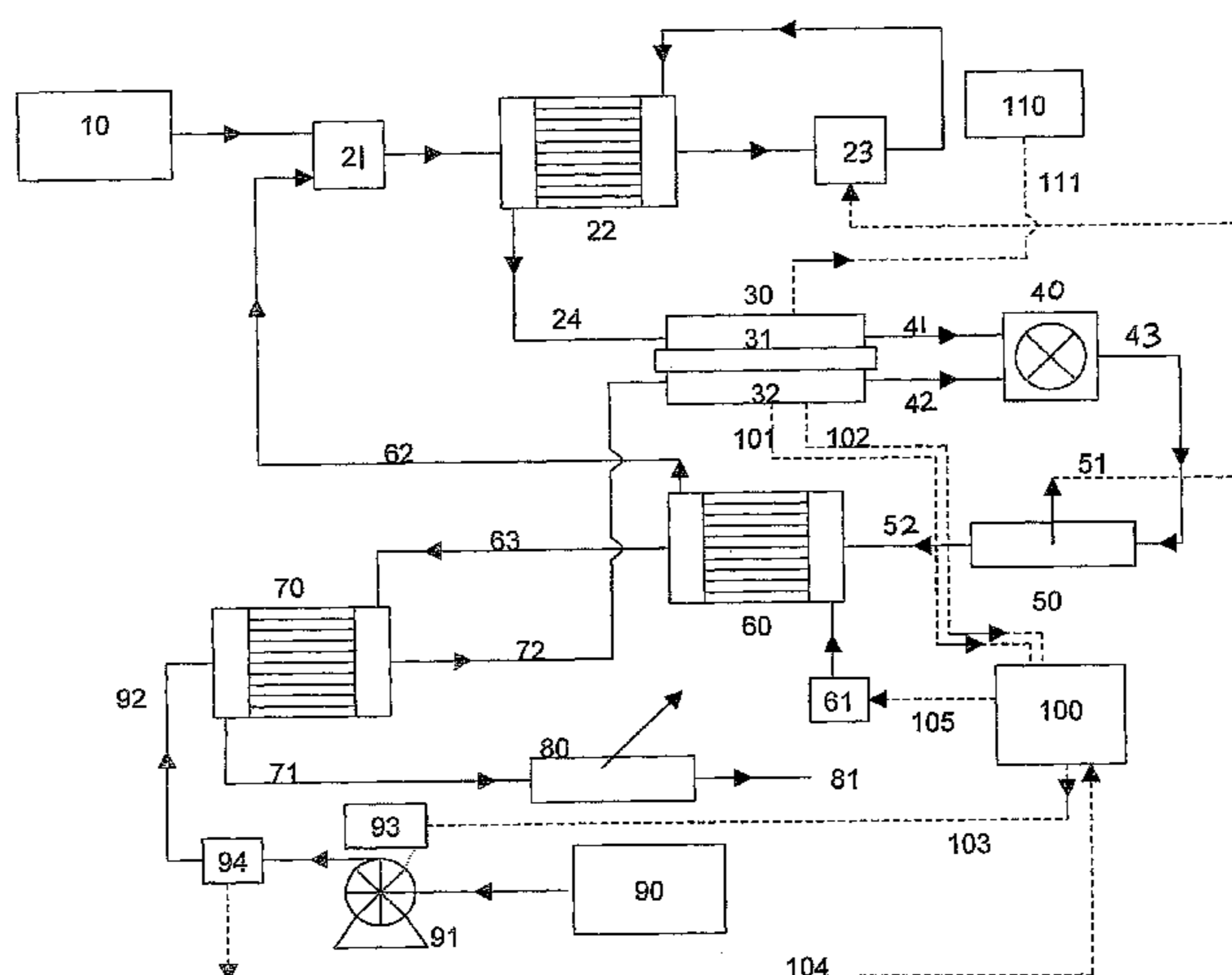
SOFC system operating on LPG showing method of implementation described in Method 1
