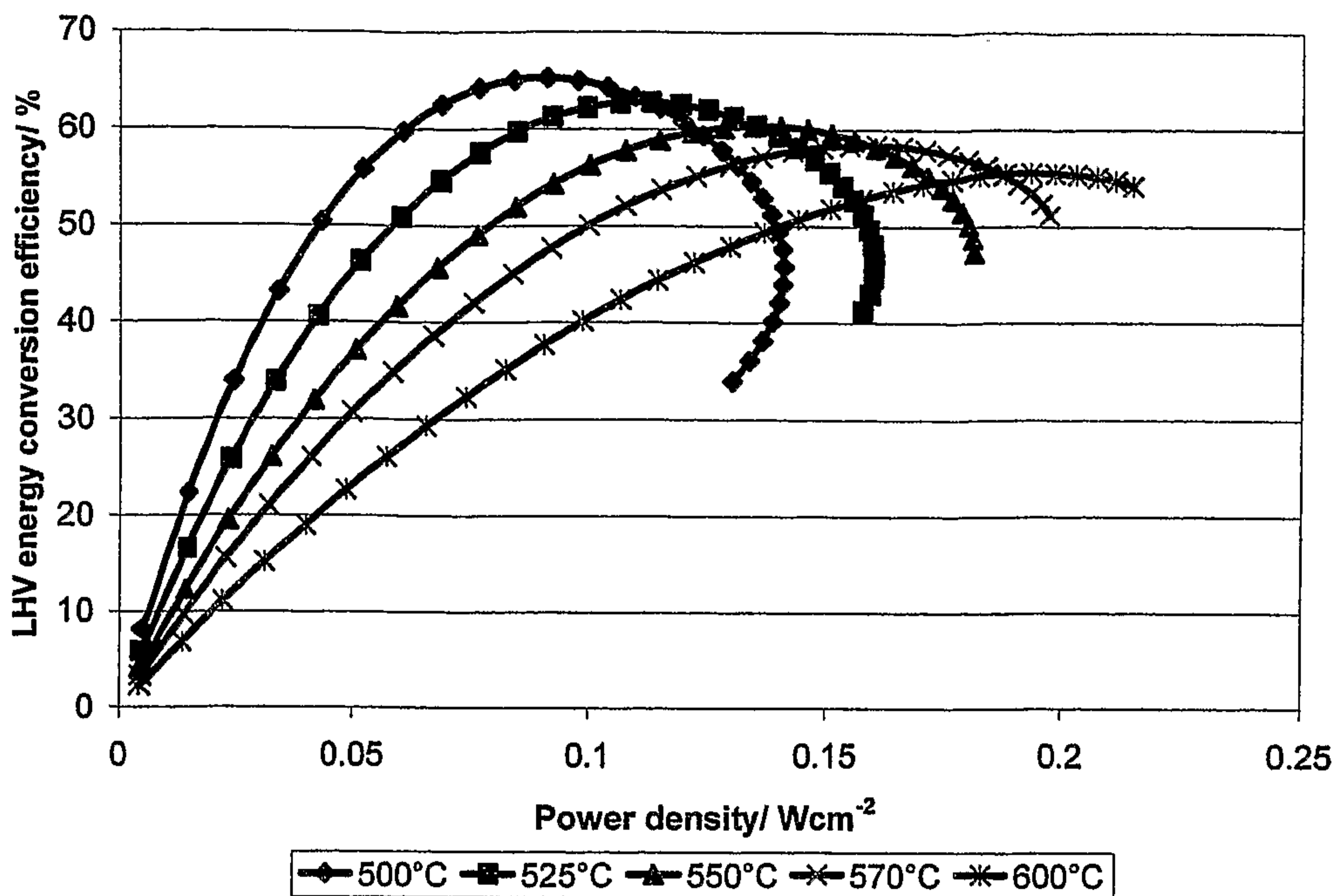
Figure 1 – LHV energy conversion efficiency as a function of electrical power density for a range of given operating temperatures
