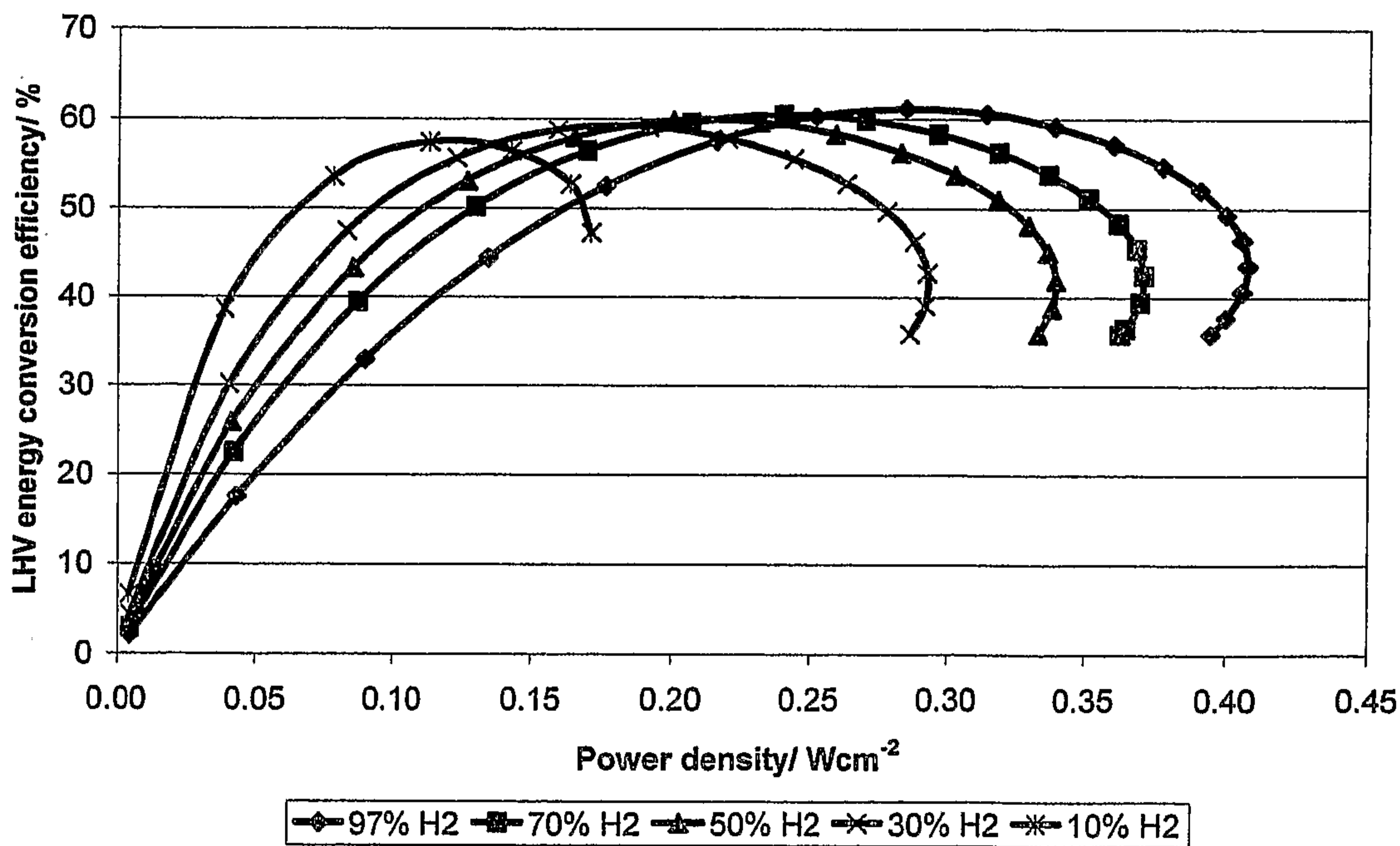
Figure 2 – LHV energy conversion efficiency as a function of electrical power density for a range of hydrogen % in steam
