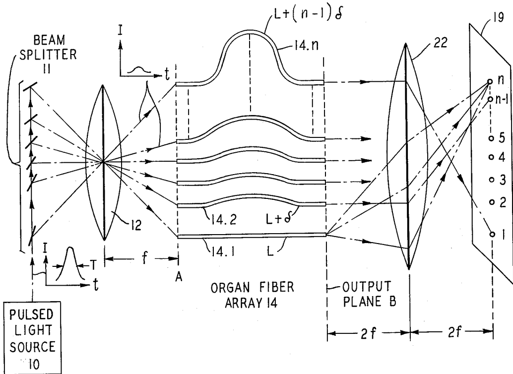
FIG. 1 PASSIVE LINE SCANNER
