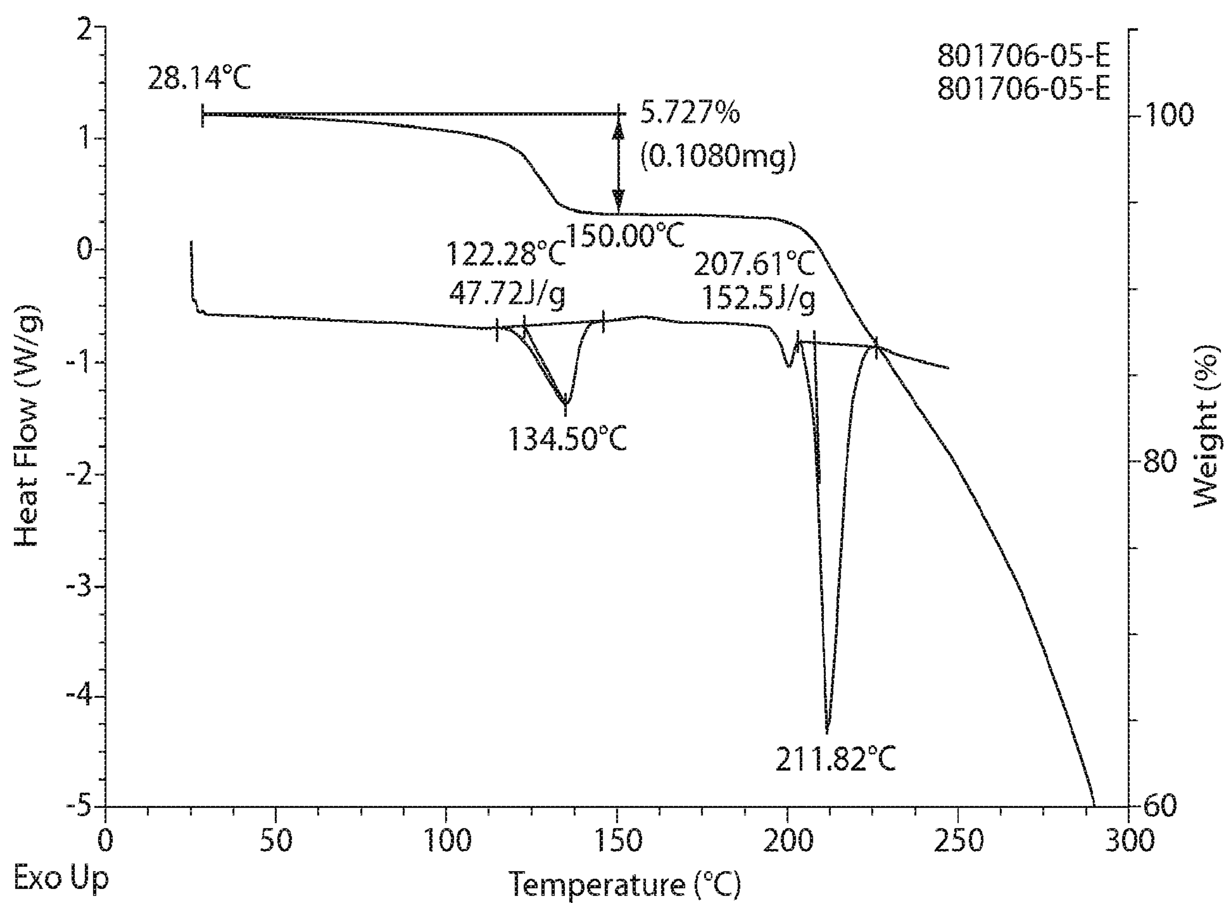
DSC and TGA profile of Form 14
