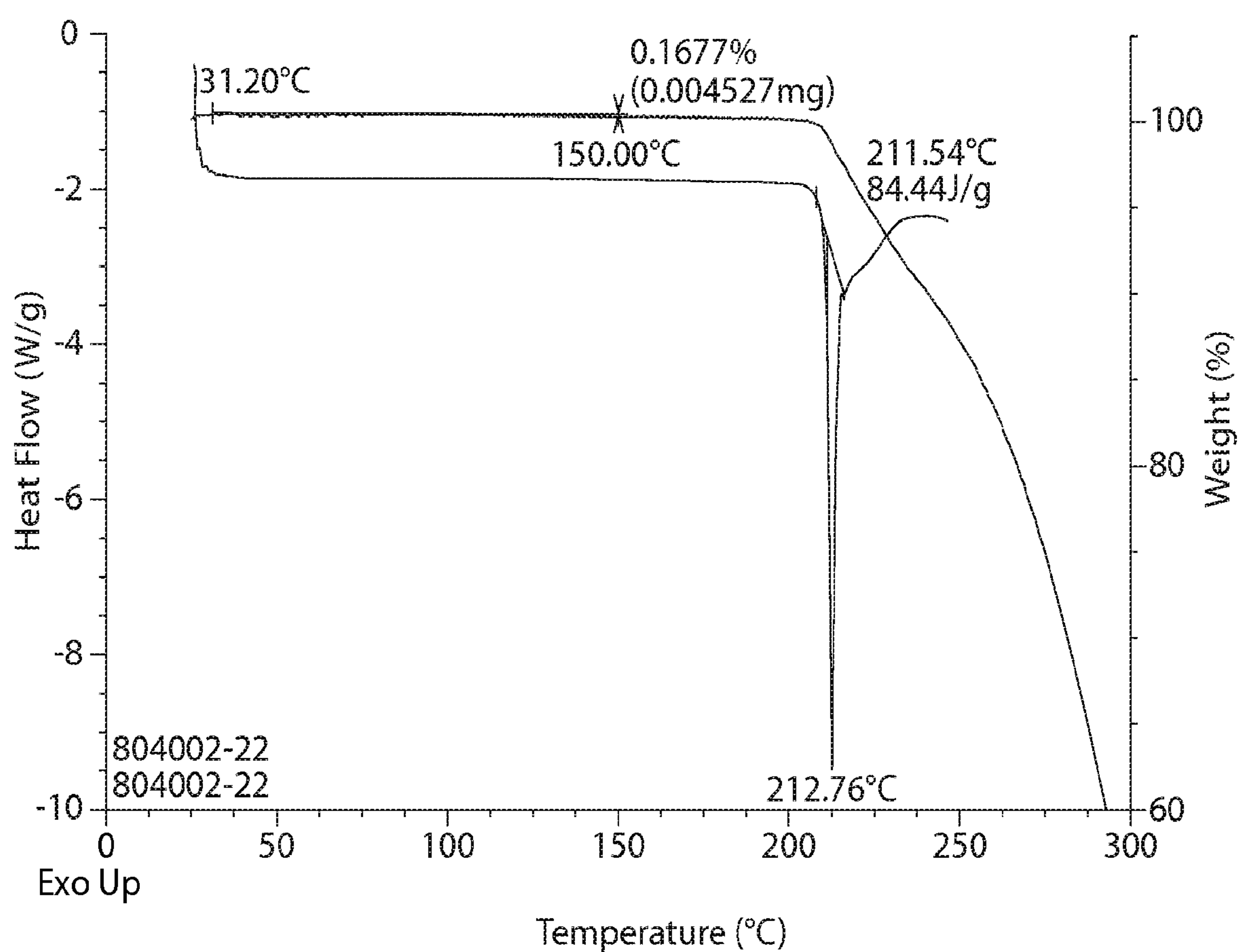
DSC and TGA profile of Form 8
