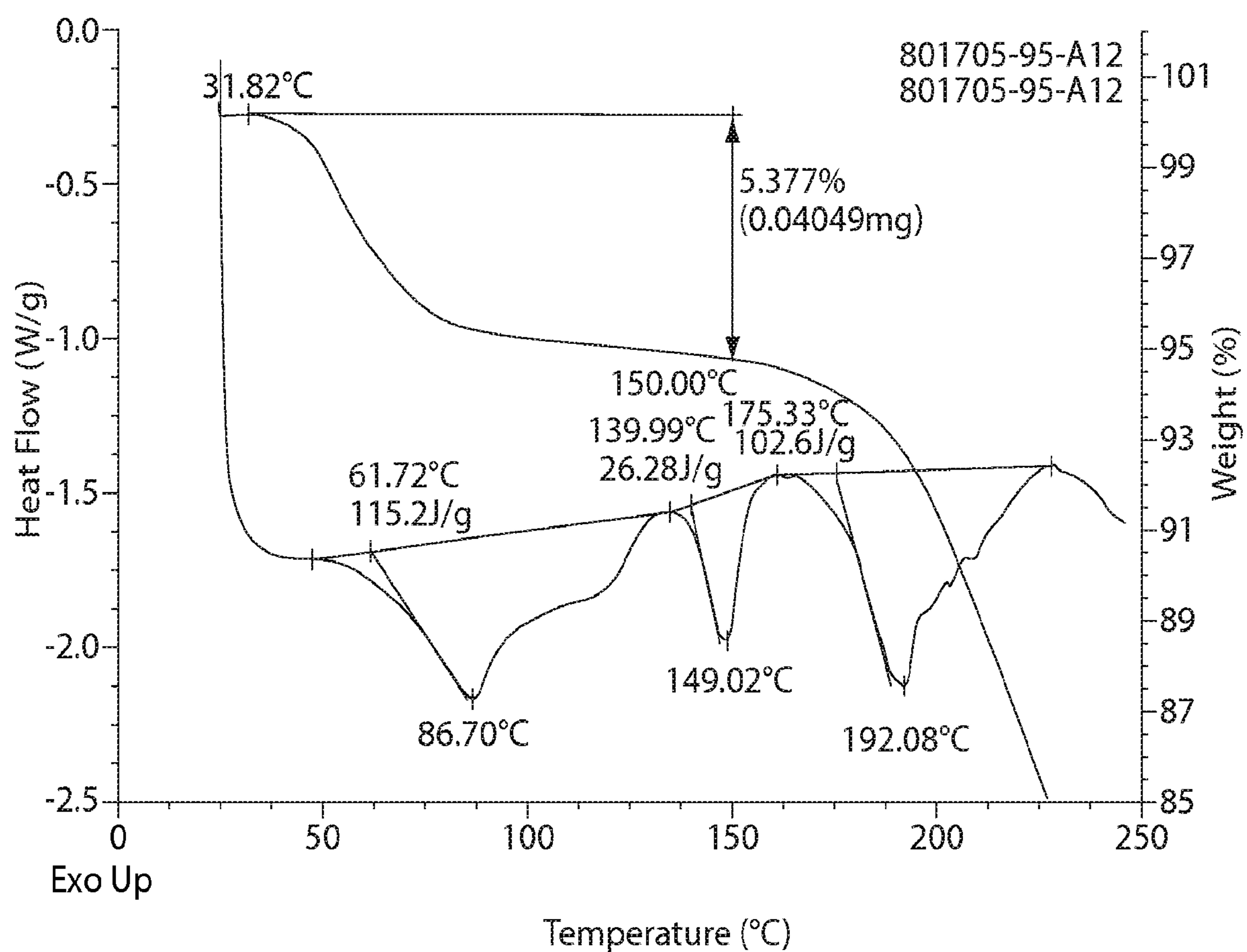
DSC and TGA profile of Form 6
