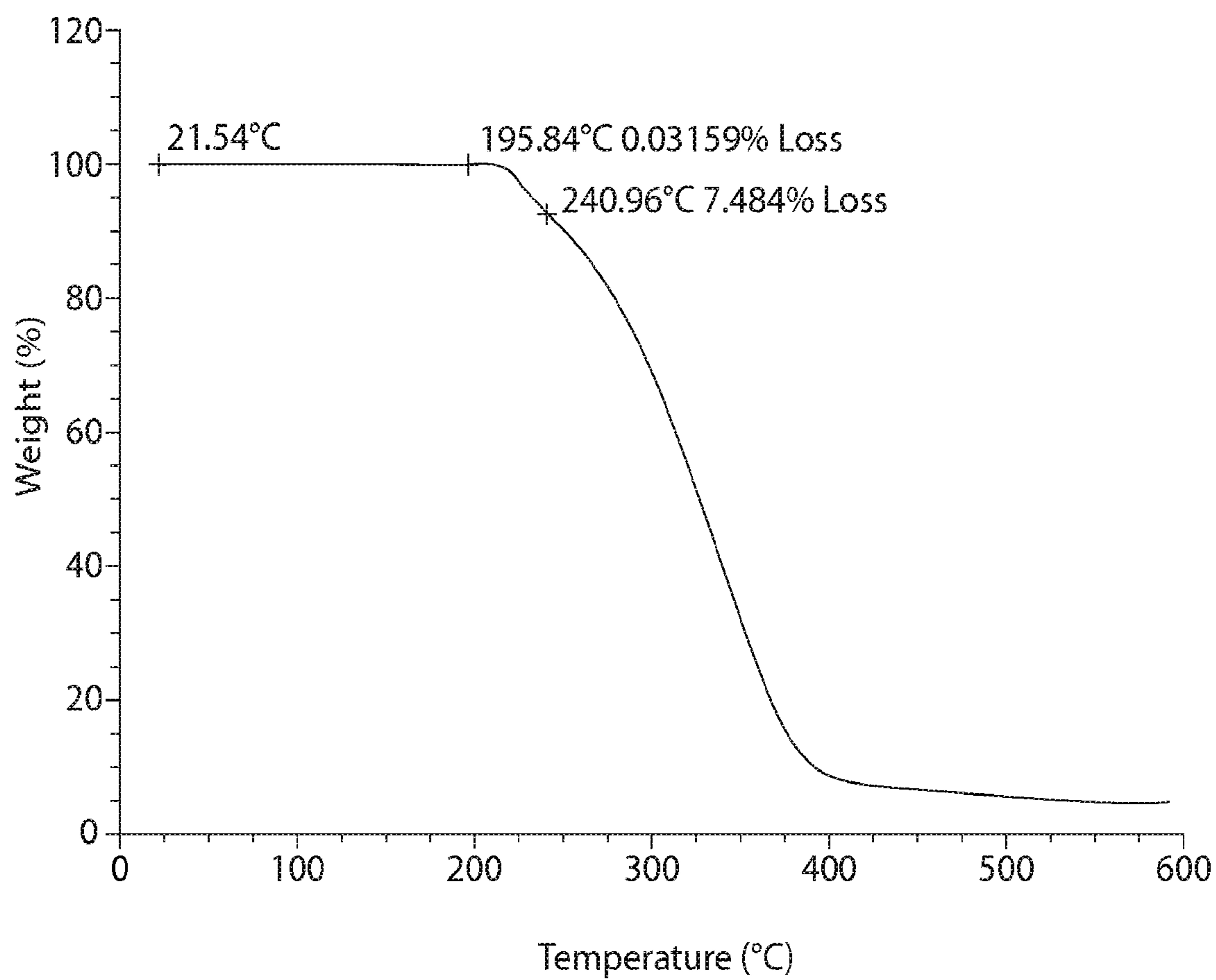
TGA profile of Form 3
