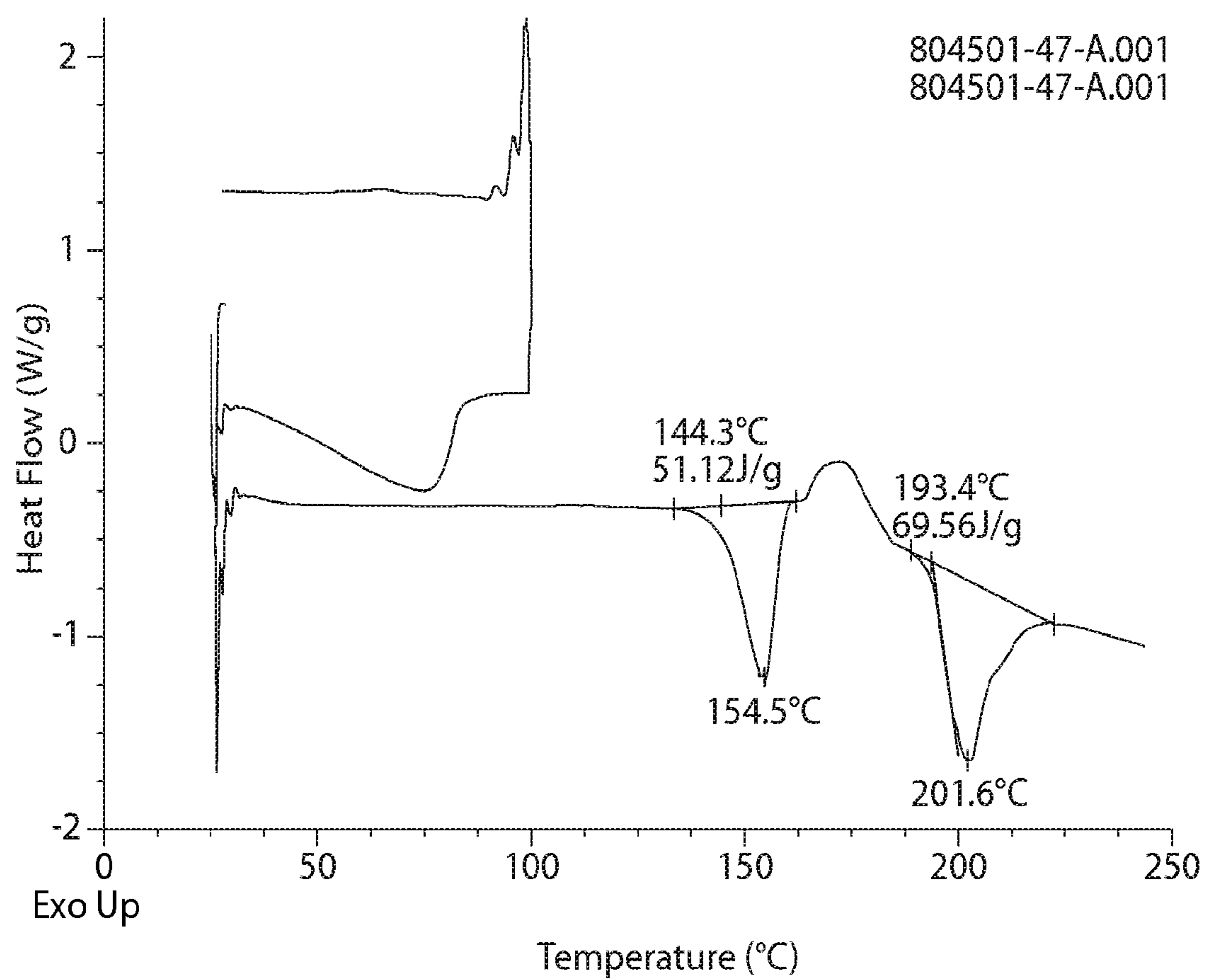
DSC and TGA profile of Form 11
