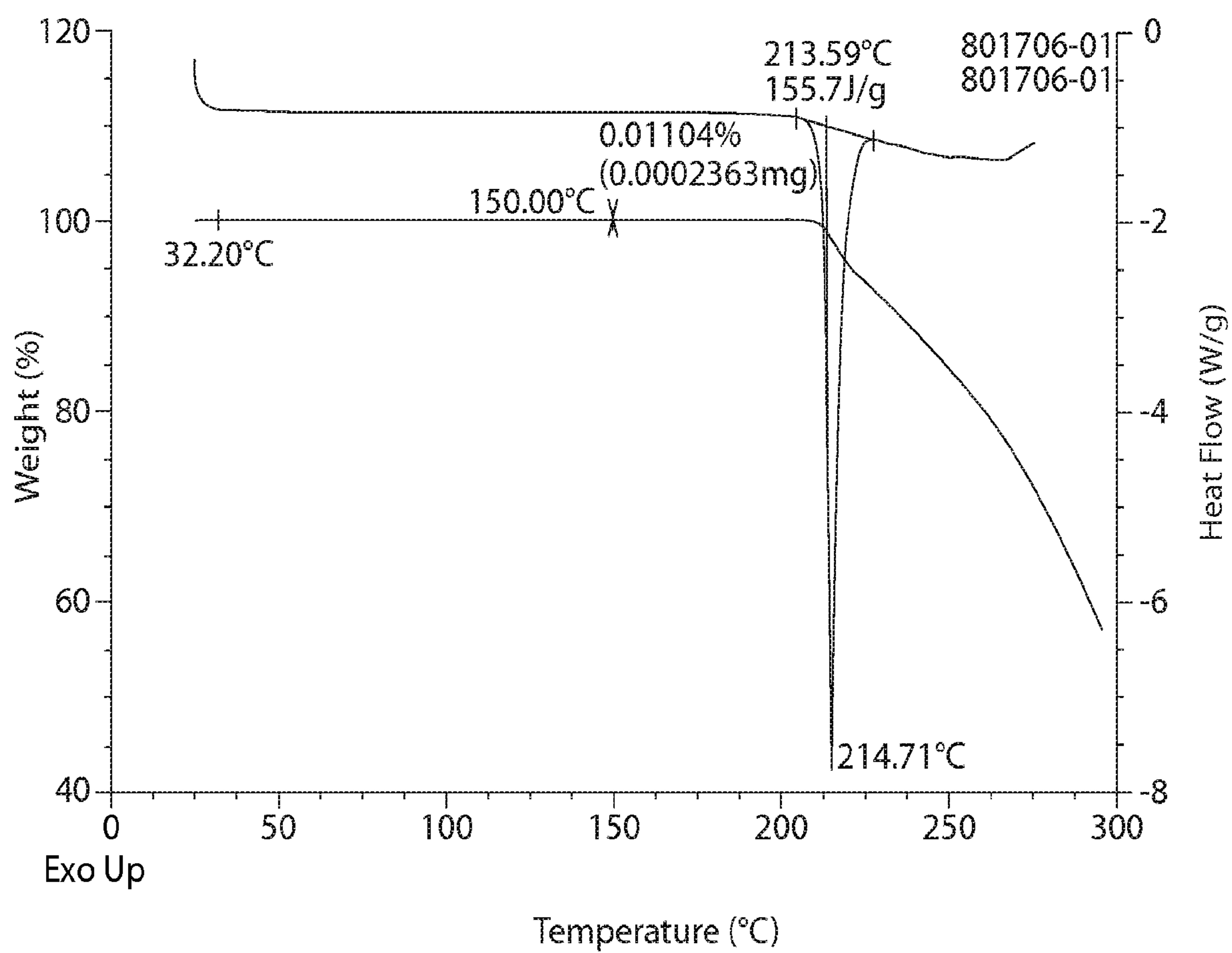
DSC and TGA profile of Form 7
