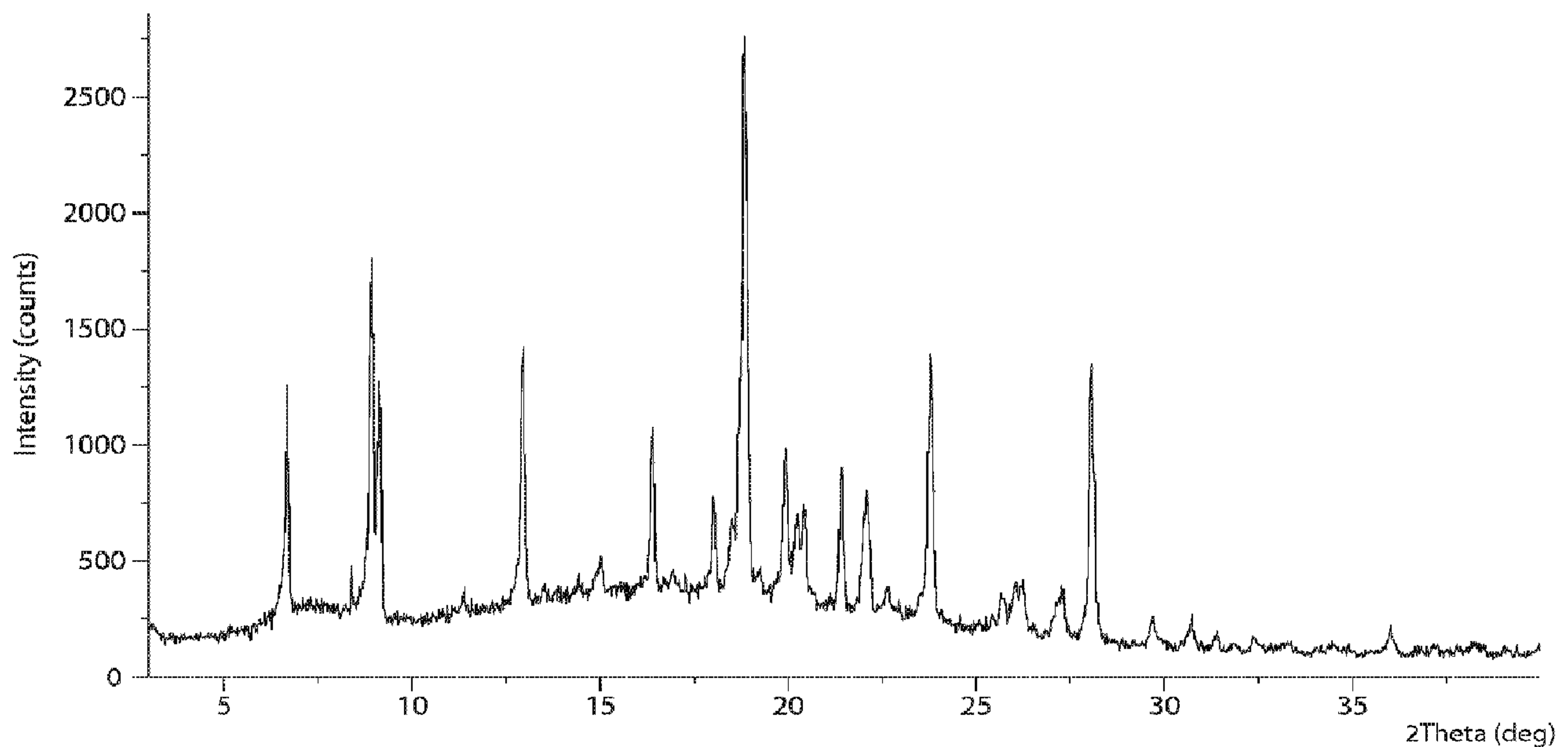
XRPD pattern of Form 1
