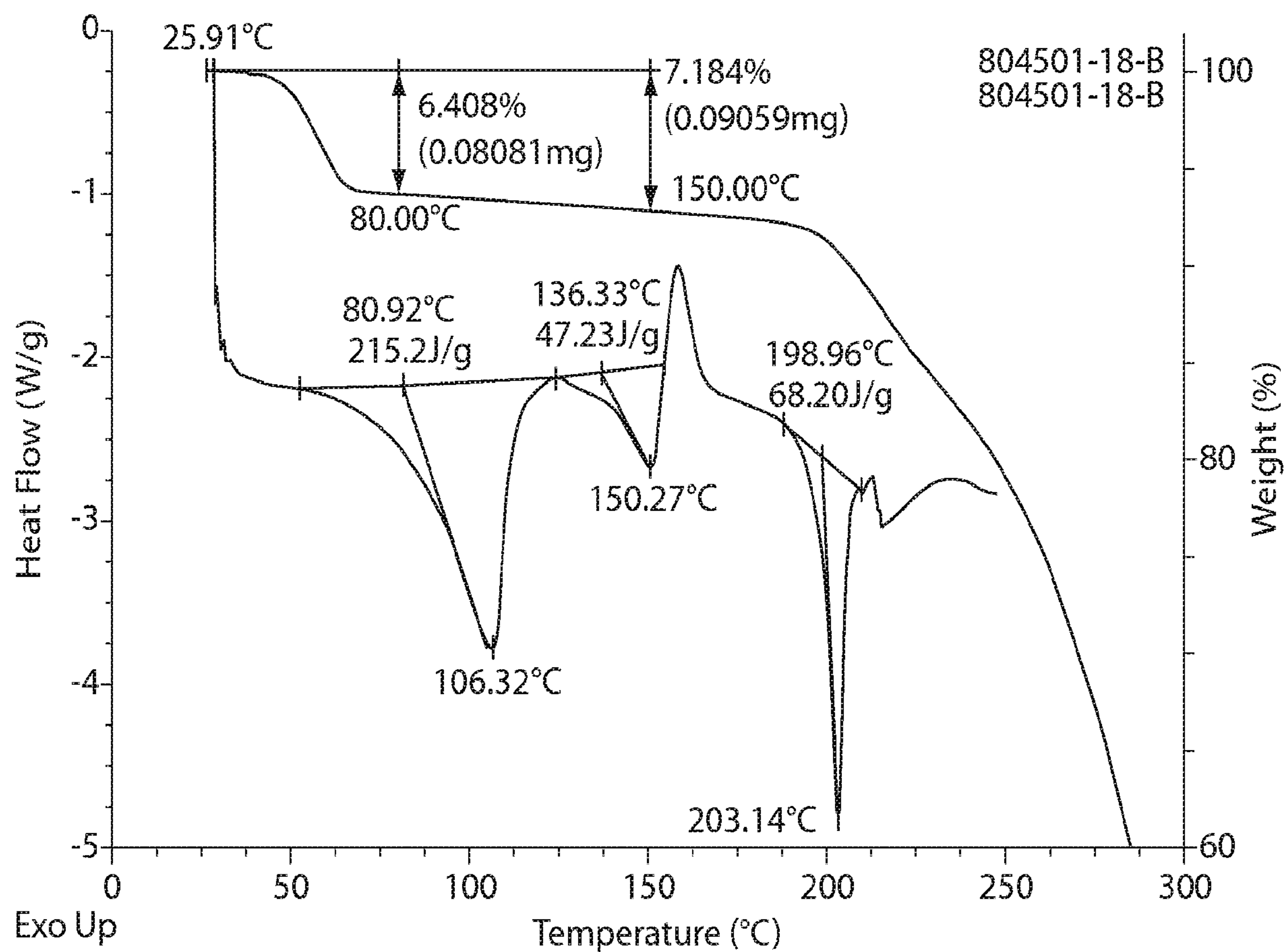
DSC and TGA profile of Form 12
