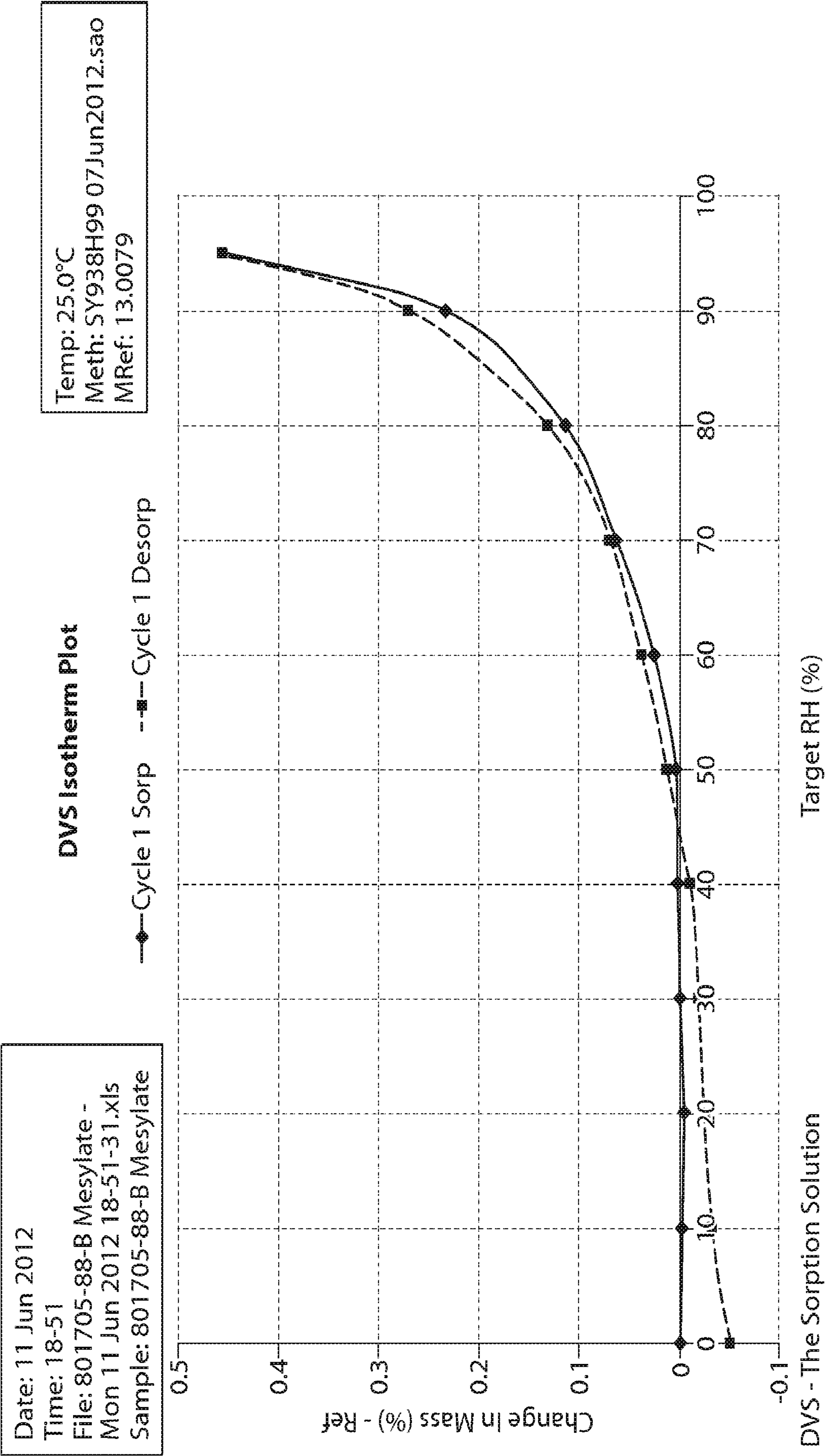
DVS profile of Form 3
