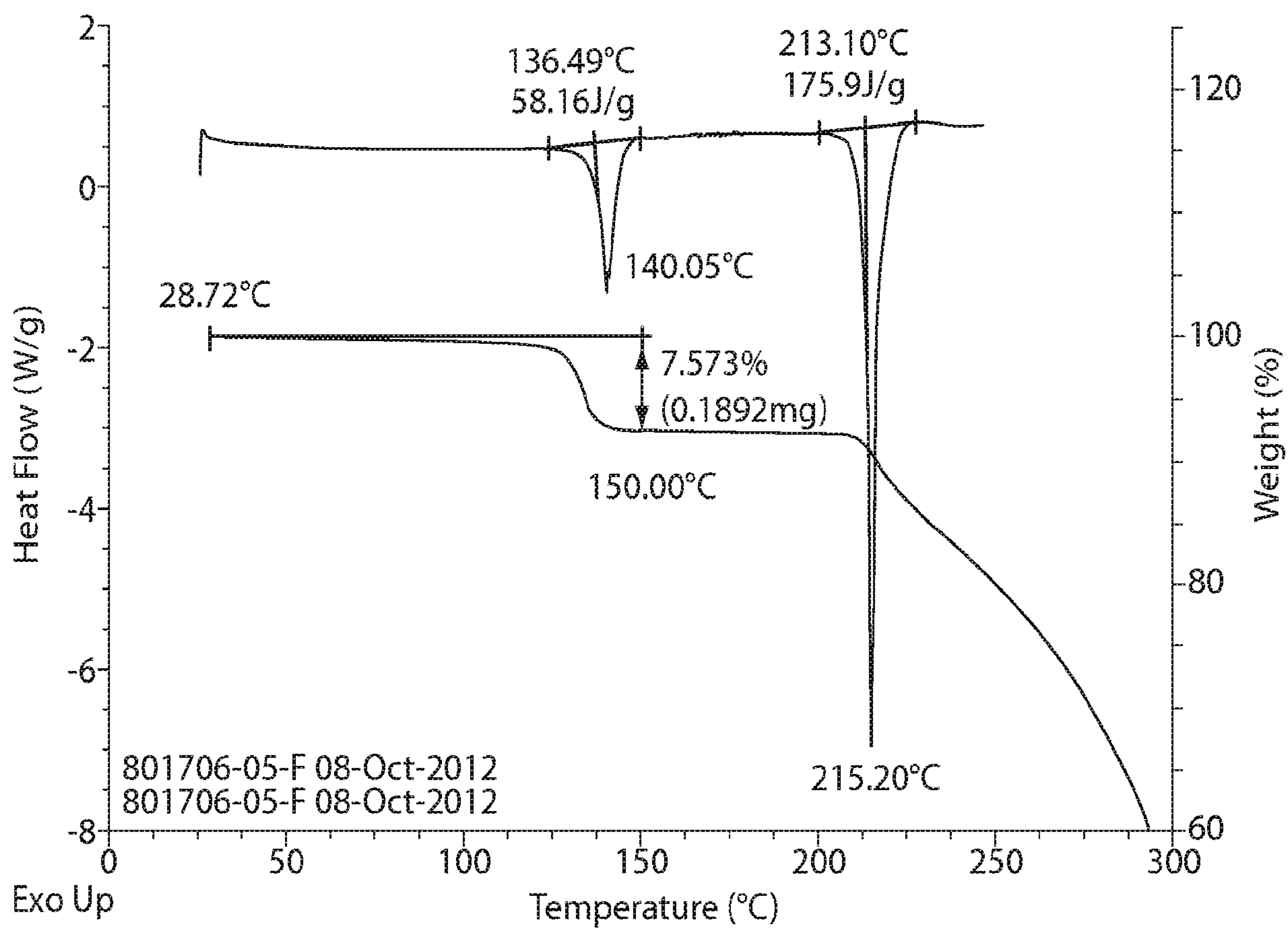
DSC and TGA profile of Form 15
