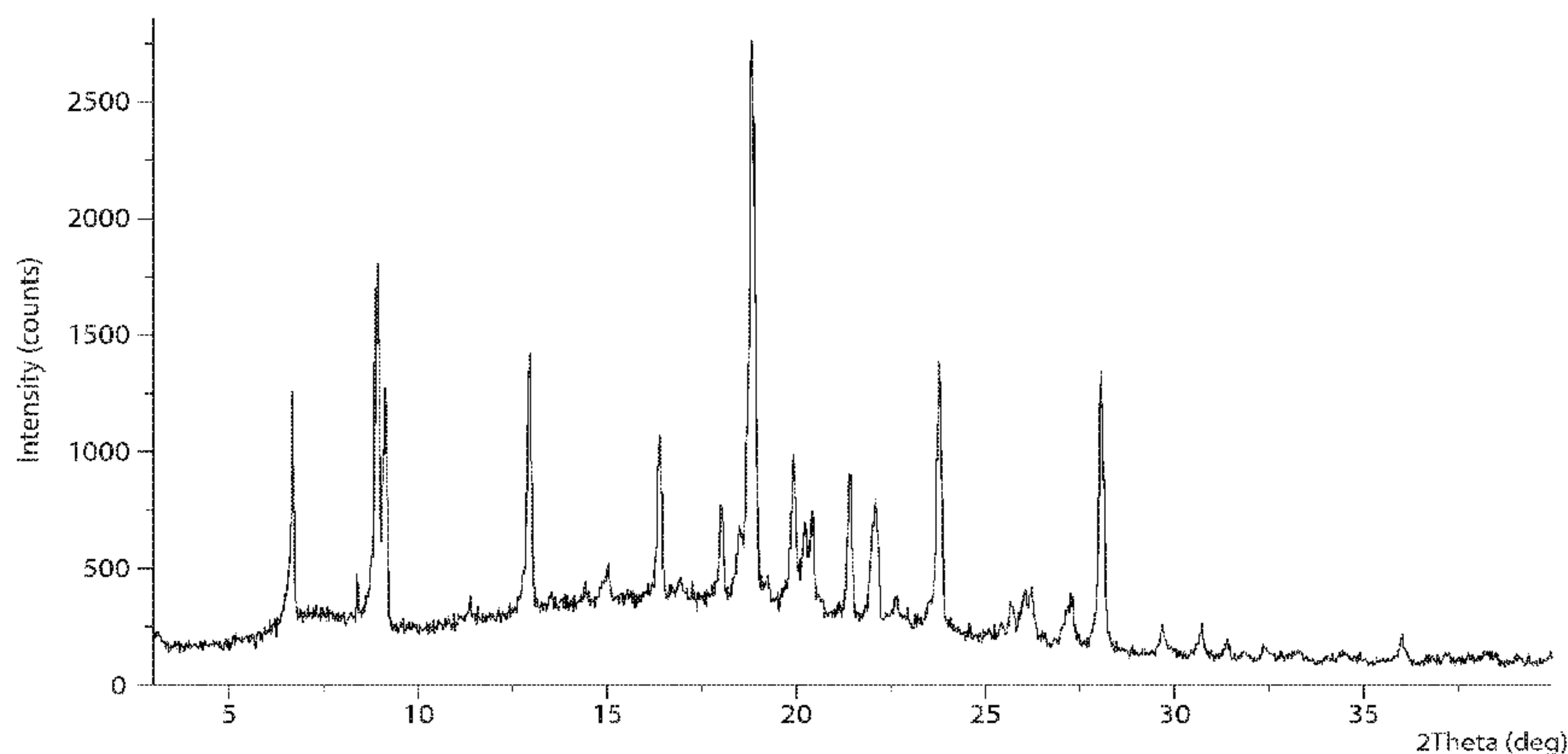
XRPD pattern of Form 1
