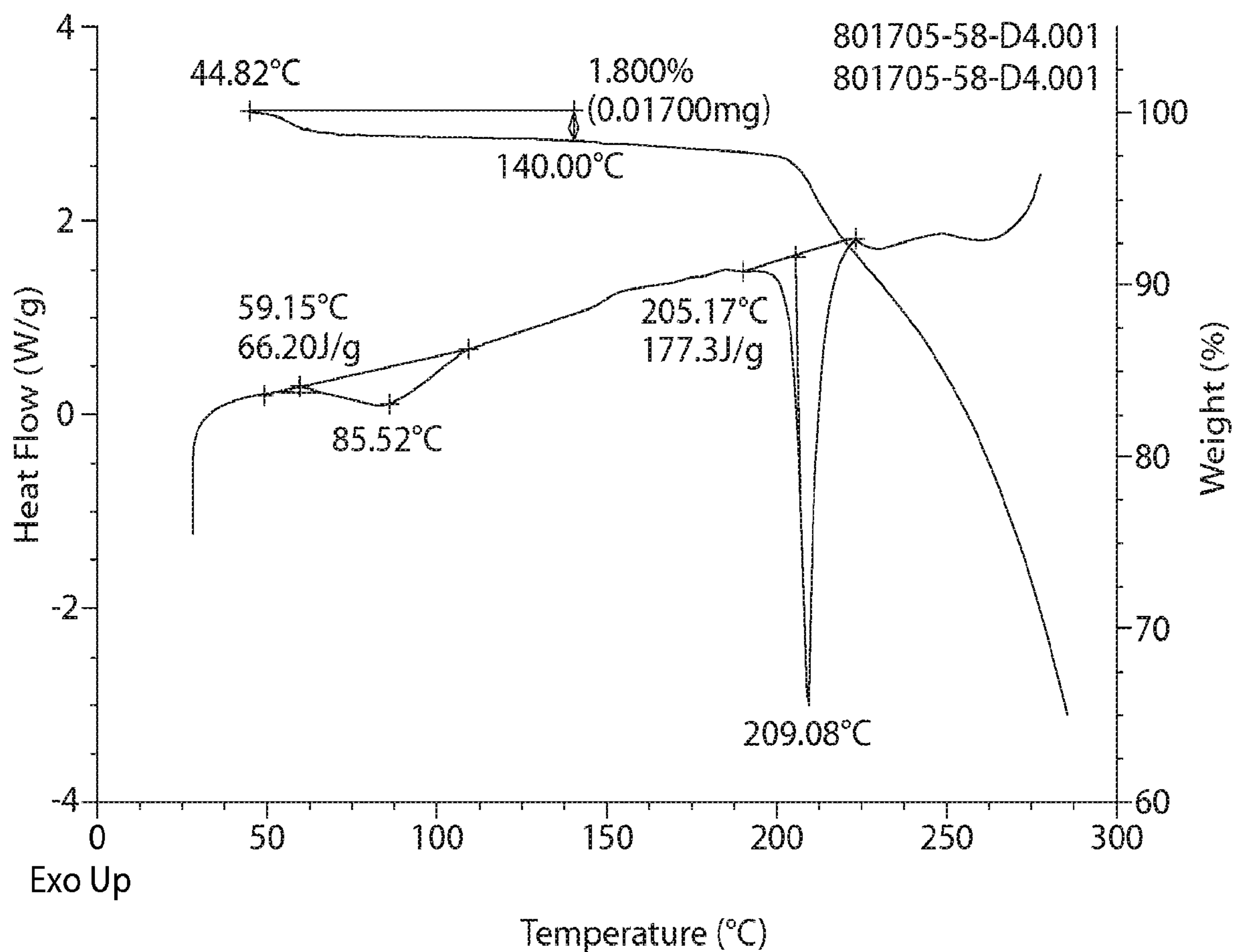
DSC and TGA profile of Form 4
