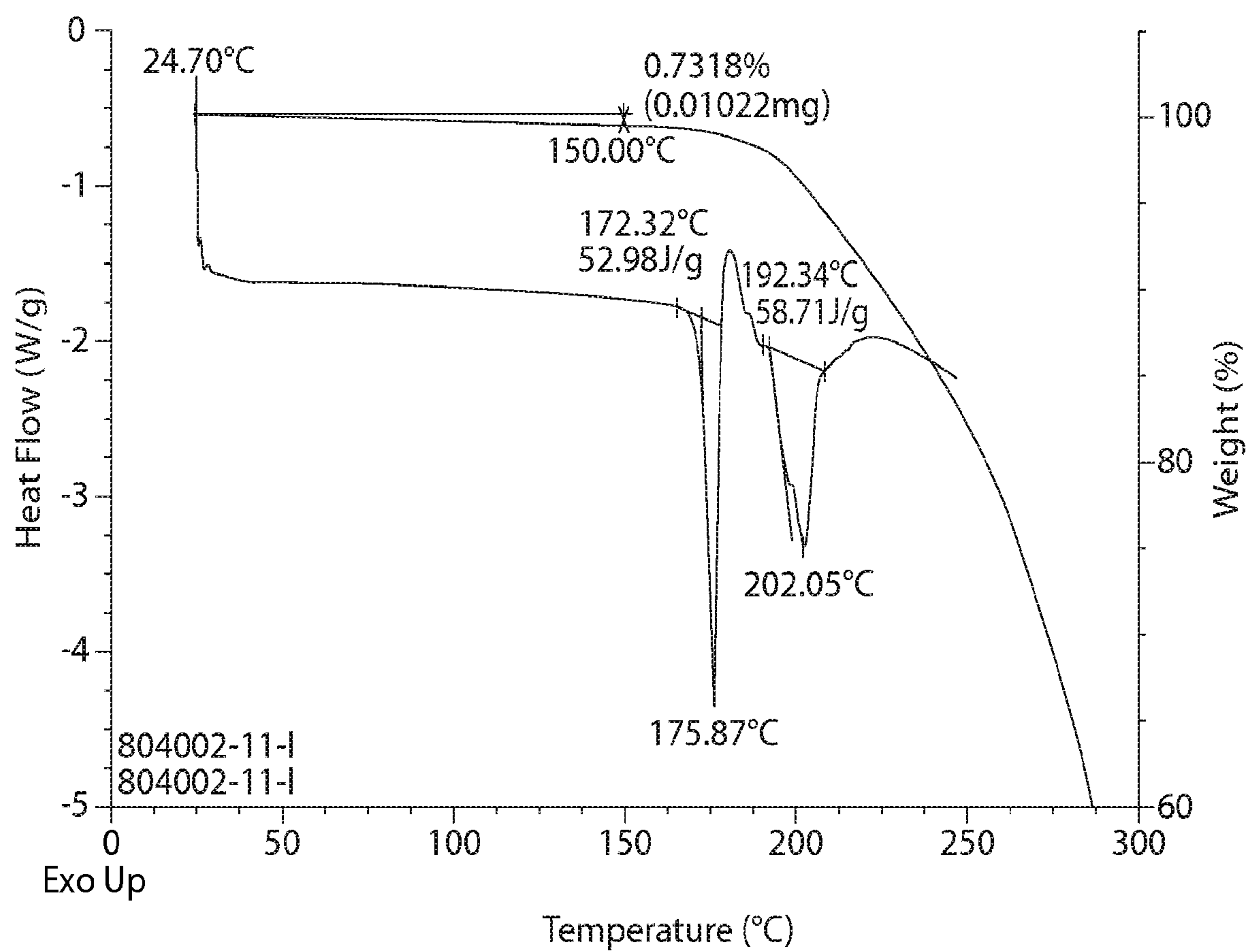
DSC and TGA profile of Form 9
