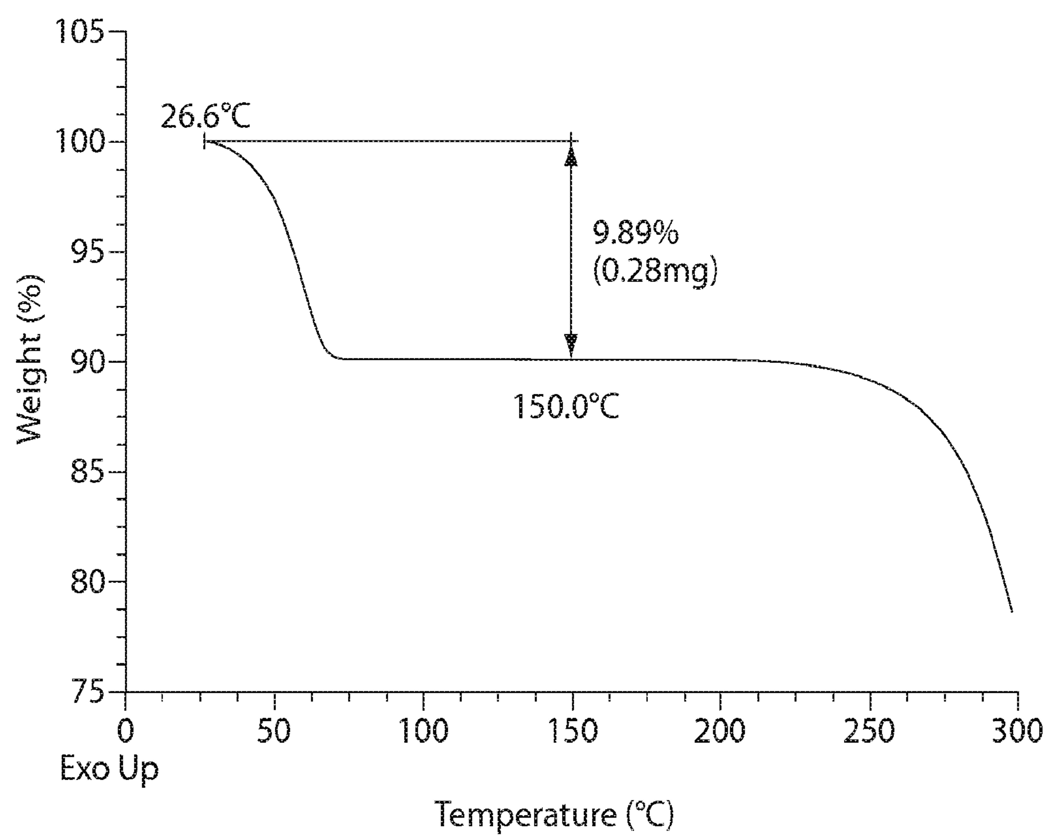
TGA profile of Form 2
