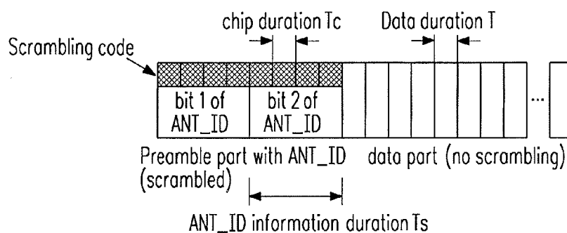
Fig. 6: Example of scrambling on beacon (Spreading factor = 4 for Preamble part)
