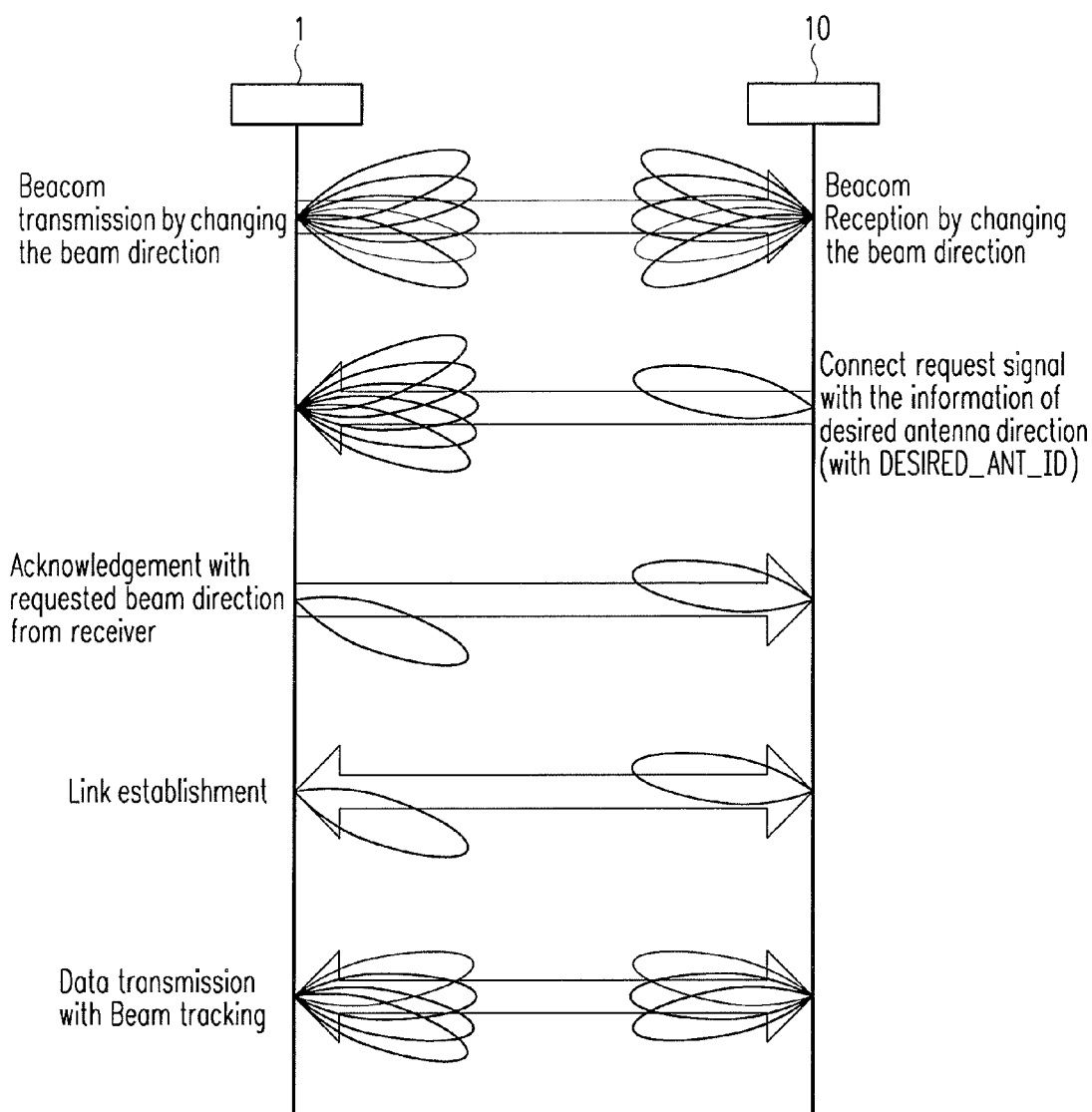
Fig. 5: Sequence chart of the invention
