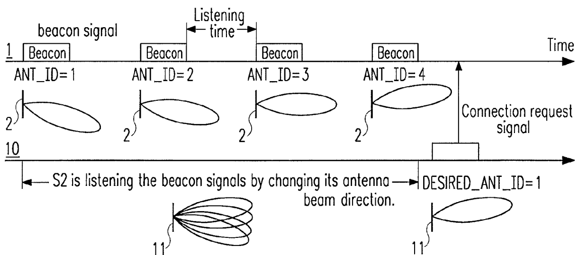
Fig. 4 : Example of initial sequence (Beacon transmission and connection request signal)
