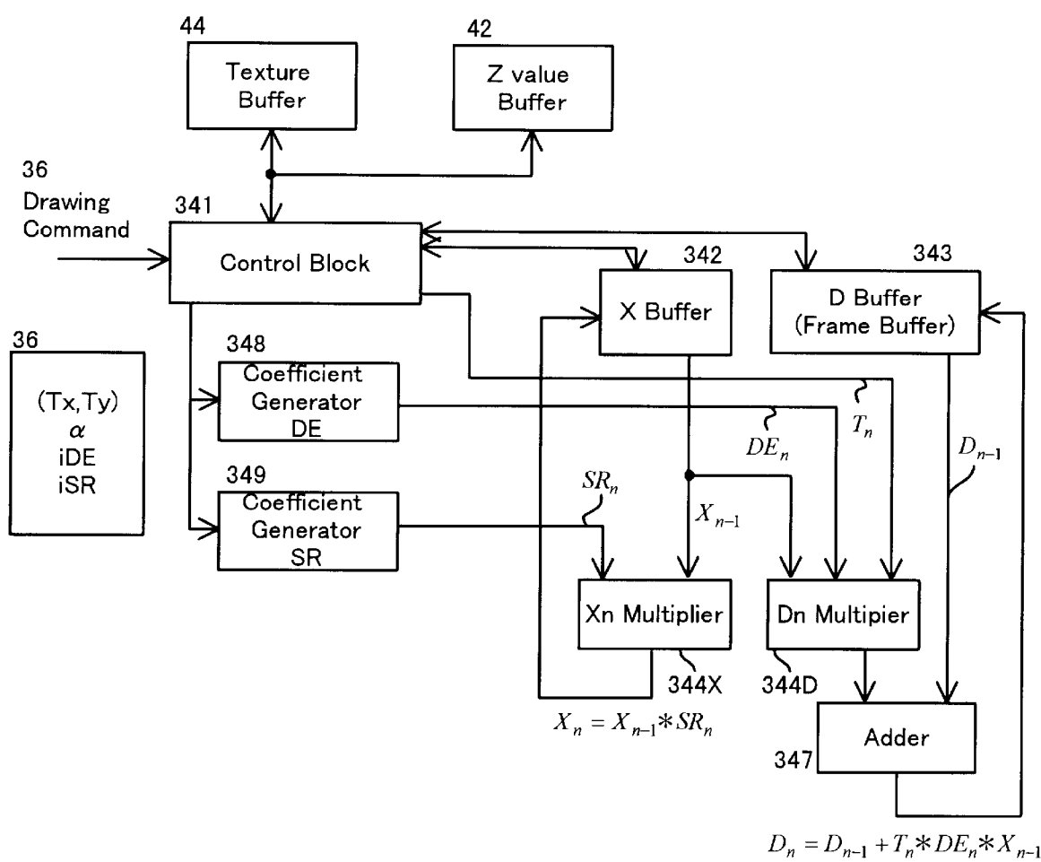
FIG. 10 General Renderer
