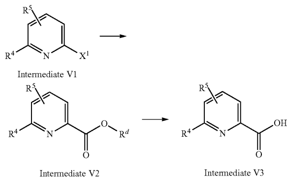
Synthesis Scheme 1
