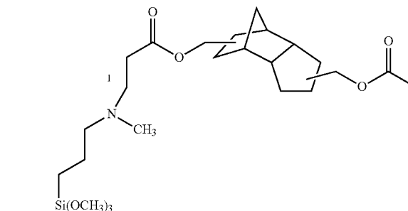
+ 9 SR 833s Michael Adduct 2 in SR 833s
