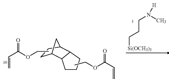
SR 833s
