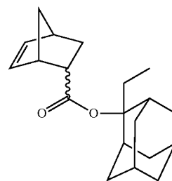
2-ethyladamantan-2-yl bicyclo[2.2.1]hept-5-ene-2-carboxylate (EtAdEsNB);
