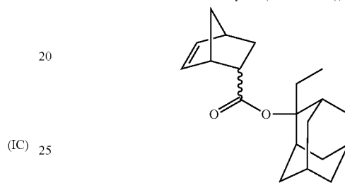
2-ethyladamantan-2-yl bicyclo[2.2.1]hept-5-ene-2-carboxylate (EtAdEsNB).
