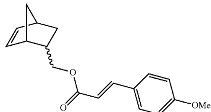
(bicyclo[2.2.1]hept-5-en-2-yl)methyl 3-(4-methoxyphenyl)acrylate (NBMeOCinnamate); and
