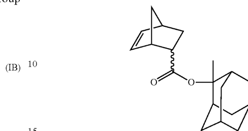
2-methyladamantan-2-yl bicyclo[2.2.1]hept-5-ene-2-carboxylate (MeAdEsNB); and
