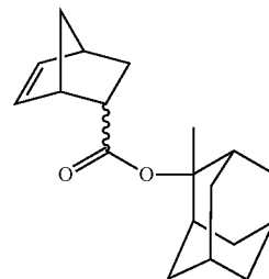
2-methyladamantan-2-yl bicyclo[2.2.1]hept-5-ene-2-carboxylate (MeAdEsNB);
