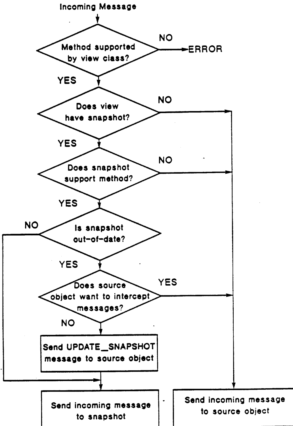
Figure 2-9. How Views Deal with Incoming Messages
