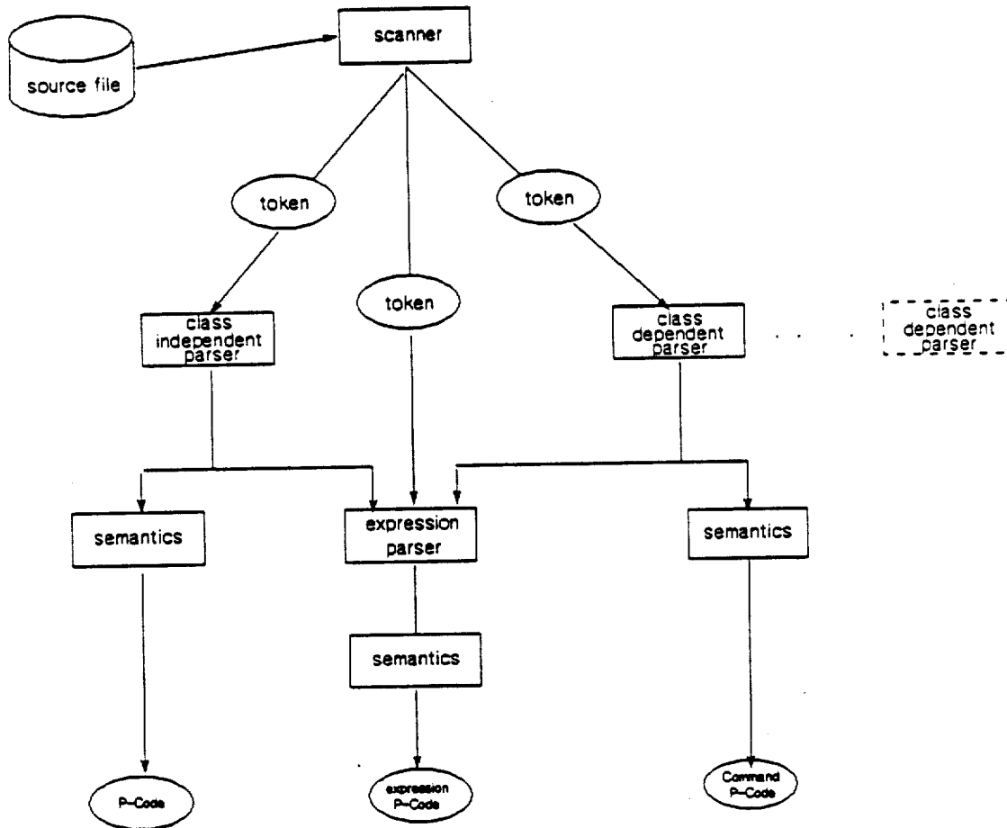
Figure 4. Parser Data Flow
