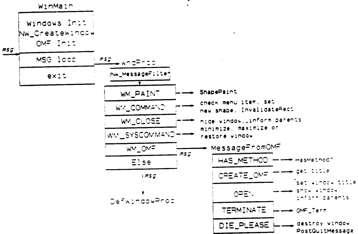
Figure 3-4. HPSHAPE Logic Flow: Final Phase
