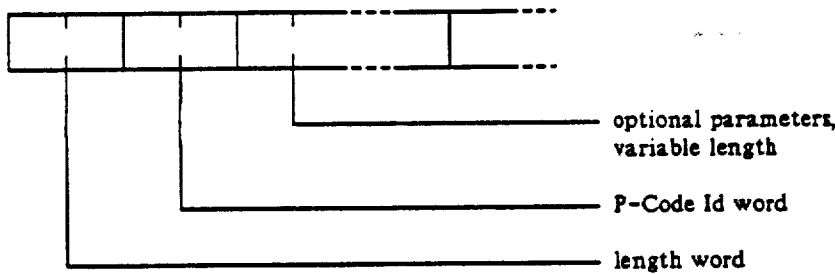
Figure 2. Binary P-Code Record Format
