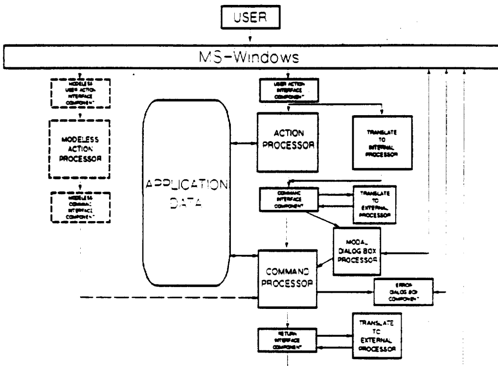
Figure 4-6. Application Architecture Block Diagram
