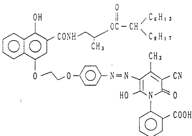
Exemplary Coupler (YC-86)
