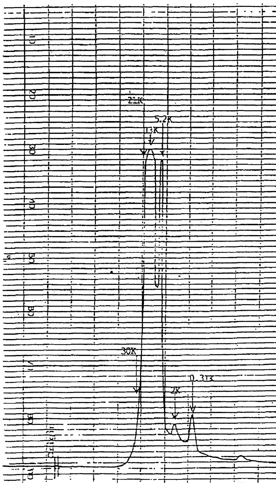
Figure 1. FPLC elution profile of the NDS as prepared by the modified method.
