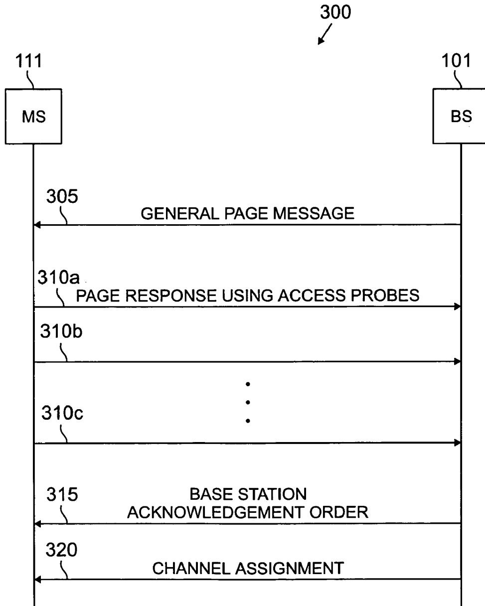
FIG. 3 (PRIOR ART)
