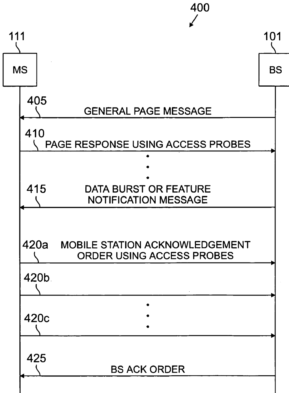
FIG. 4 (PRIOR ART)
