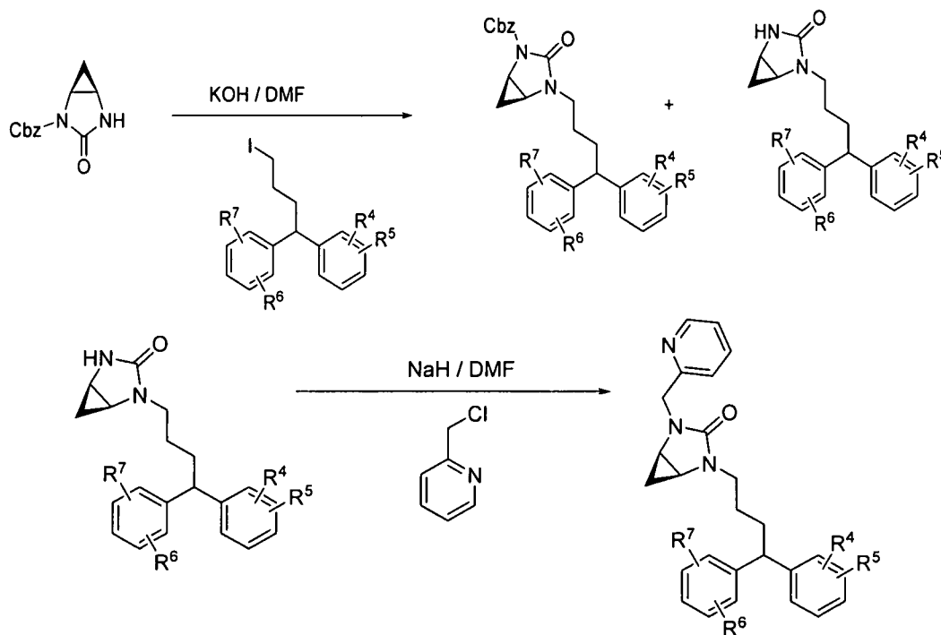
Scheme 4
