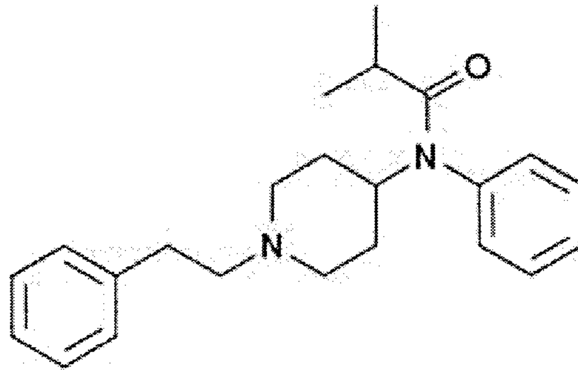
Isobutyrfentanyl
