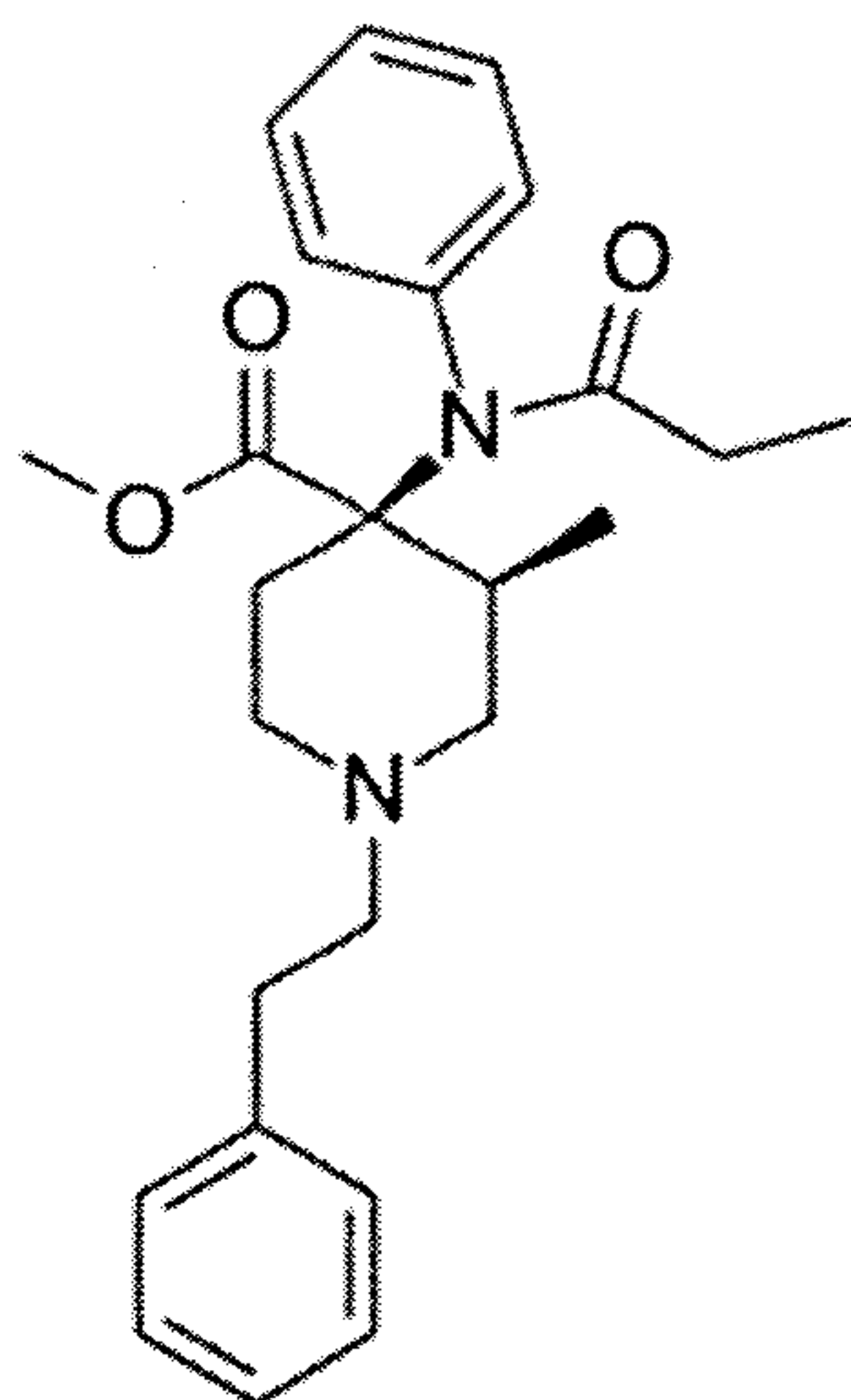
Lofentanyl
