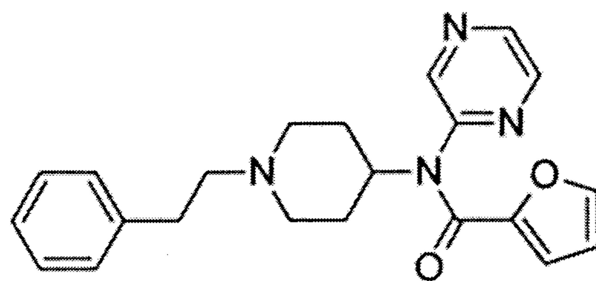
Mirfentanyl
