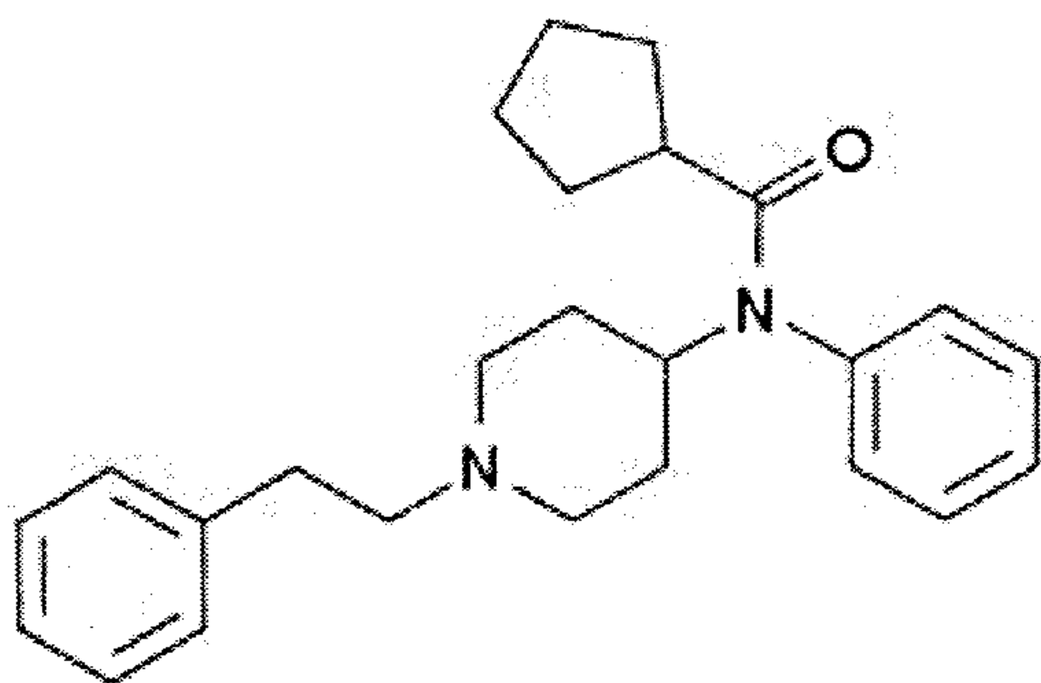
Cyclopentylfentanyl
