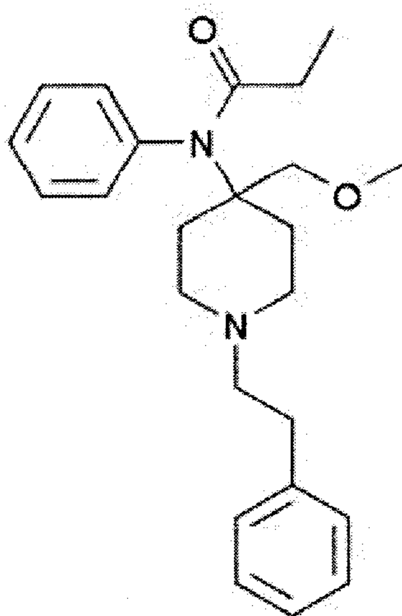
Ocfentanyl
