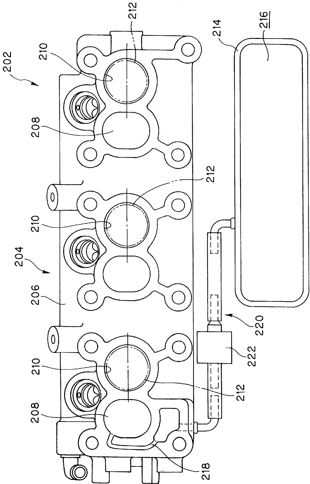
FIG. 18 (PRIOR ART)
