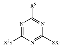
(derivative d)
