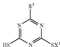
(derivative e)
