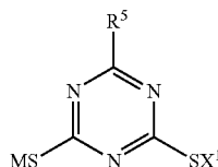
(derivative f)
