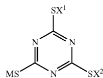
(derivative c)
