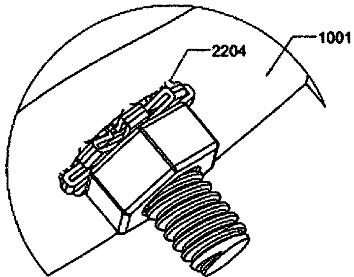
DETAIL A
