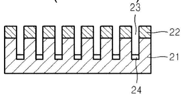
FIG. 2C (PRIOR ART)
