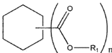
[Chemical Formula 2]
