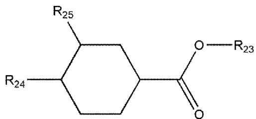
[Chemical Formula 2-5]
