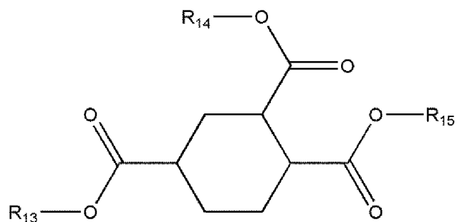
[Chemical Formula 1-3]
