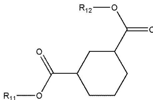
[Chemical Formula 2-2]
