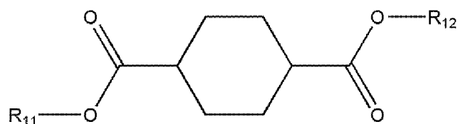
[Chemical Formula 1-1]
