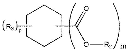
[Chemical Formula 2]
