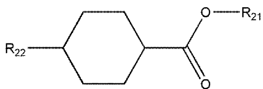
[Chemical Formula 2-2]
