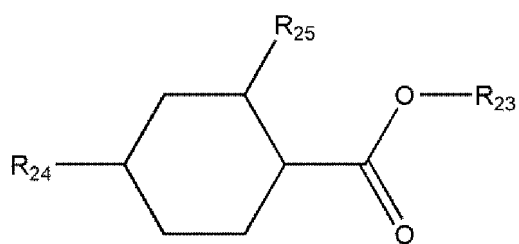
[Chemical Formula 2-7]
