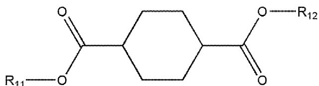
[Chemical Formula 1-1]
