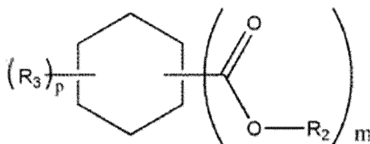
[Chemical Formula 2]
