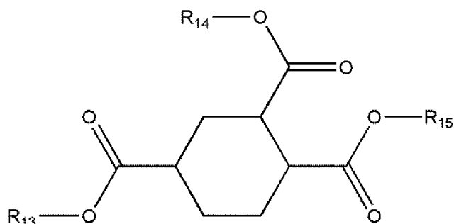
[Chemical Formula 1-3]
