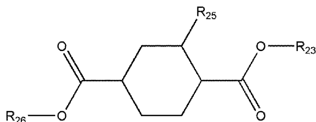
[Chemical Formula 2-9]
