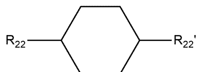
[Chemical Formula 2-3]
