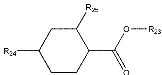
[Chemical Formula 2-7]
