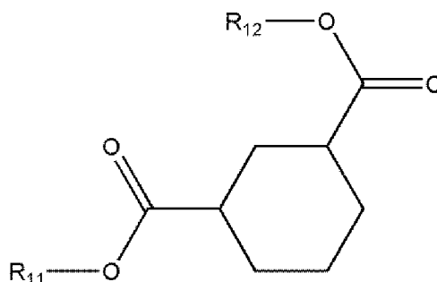
[Chemical Formula 1-3]
