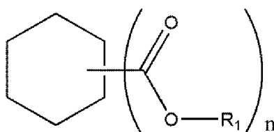
[Chemical Formula 2]
