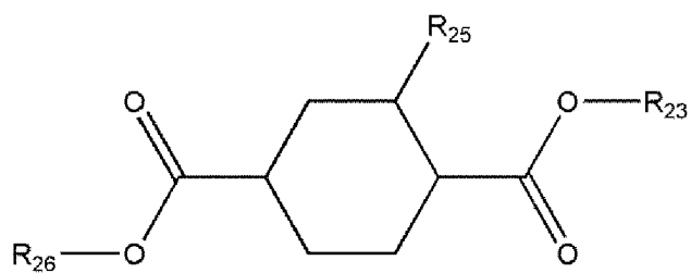
[Chemical Formula 2-9]
