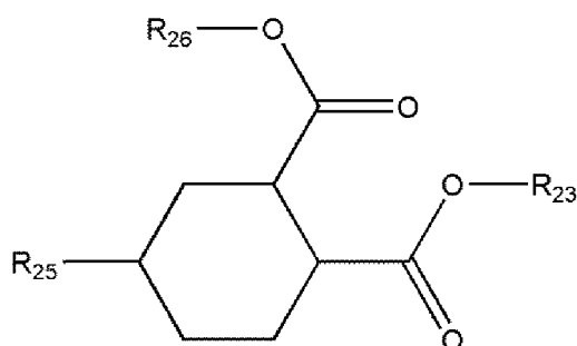
[Chemical Formula 2-10]
