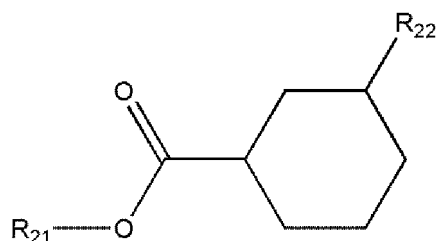
[Chemical Formula 2-2]
