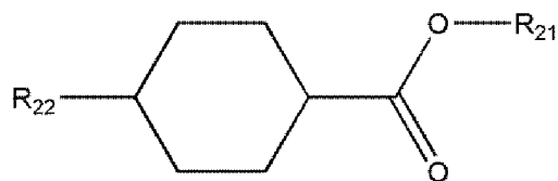
[Chemical Formula 2-1]
