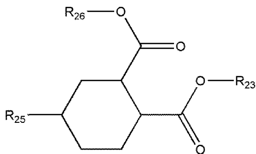
[Chemical Formula 2-9]
