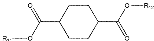
[Chemical Formula 1-2]
