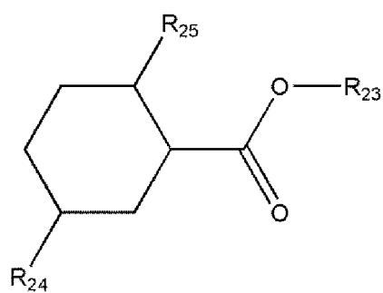
[Chemical Formula 2-8]
