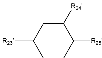
[Chemical Formula 2-11]
