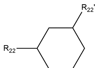
[Chemical Formula 2-5]
