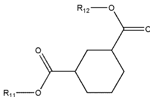
[Chemical Formula 1-3]
