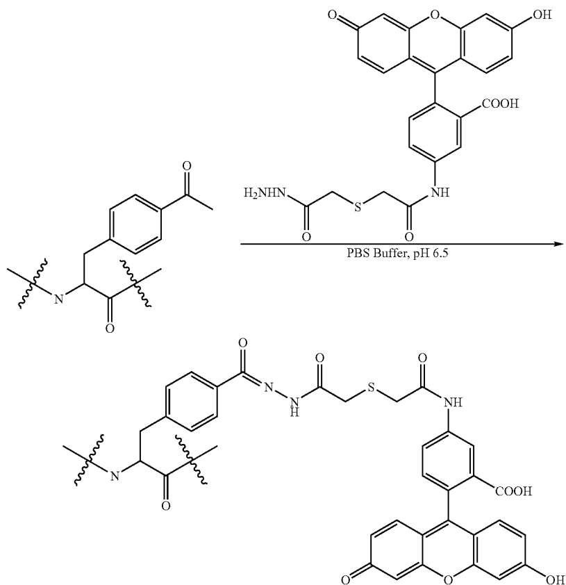
Scheme 1
