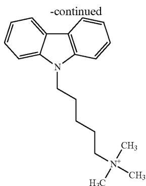
5-(9H-carbazol-9-yl)-N,N,N-trimethylpentan-1-aminium
