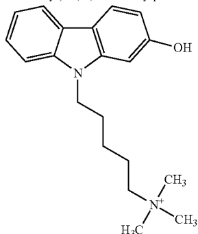
5-(2-hydroxy-9H-carbazol-9-yl)-N,N,N-trimethylpentan-1-aminium
