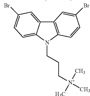
3-(3,6-dibromo-9H-carbazol-9-yl)-N,N,N-trimethylpropan-1-aminium (MTK-013)
