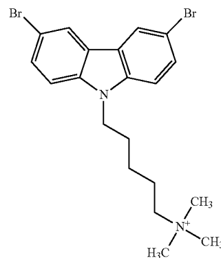
5-(3,6-dibromo-9H-carbazol-9-yl)-N,N,N-trimethylpentan-1-aminium (MTK-012)
