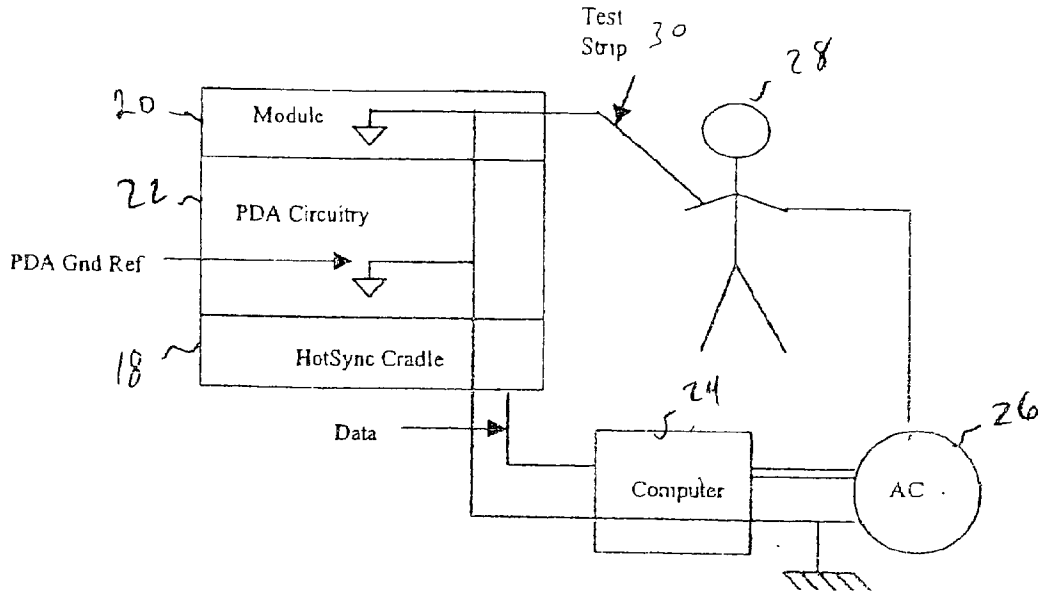
Figure 3a : PDA and Module Without Isolation
