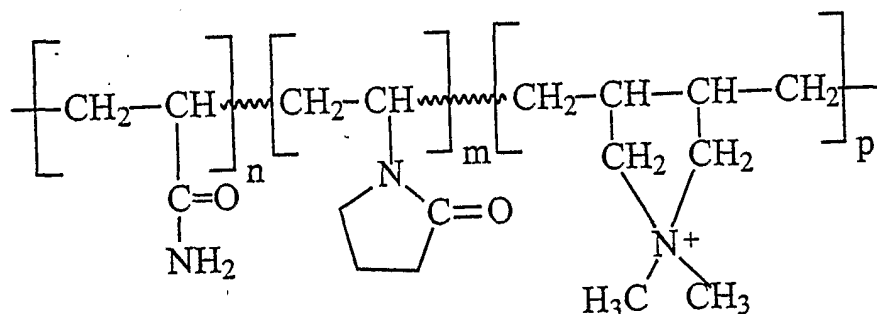
CHEMICAL STRUCTURE OF THE POLYMER DP/PT 2130
