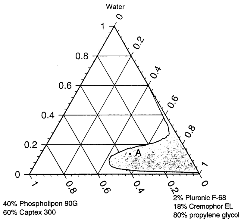
Figure 3: Ternary Phase diagram
