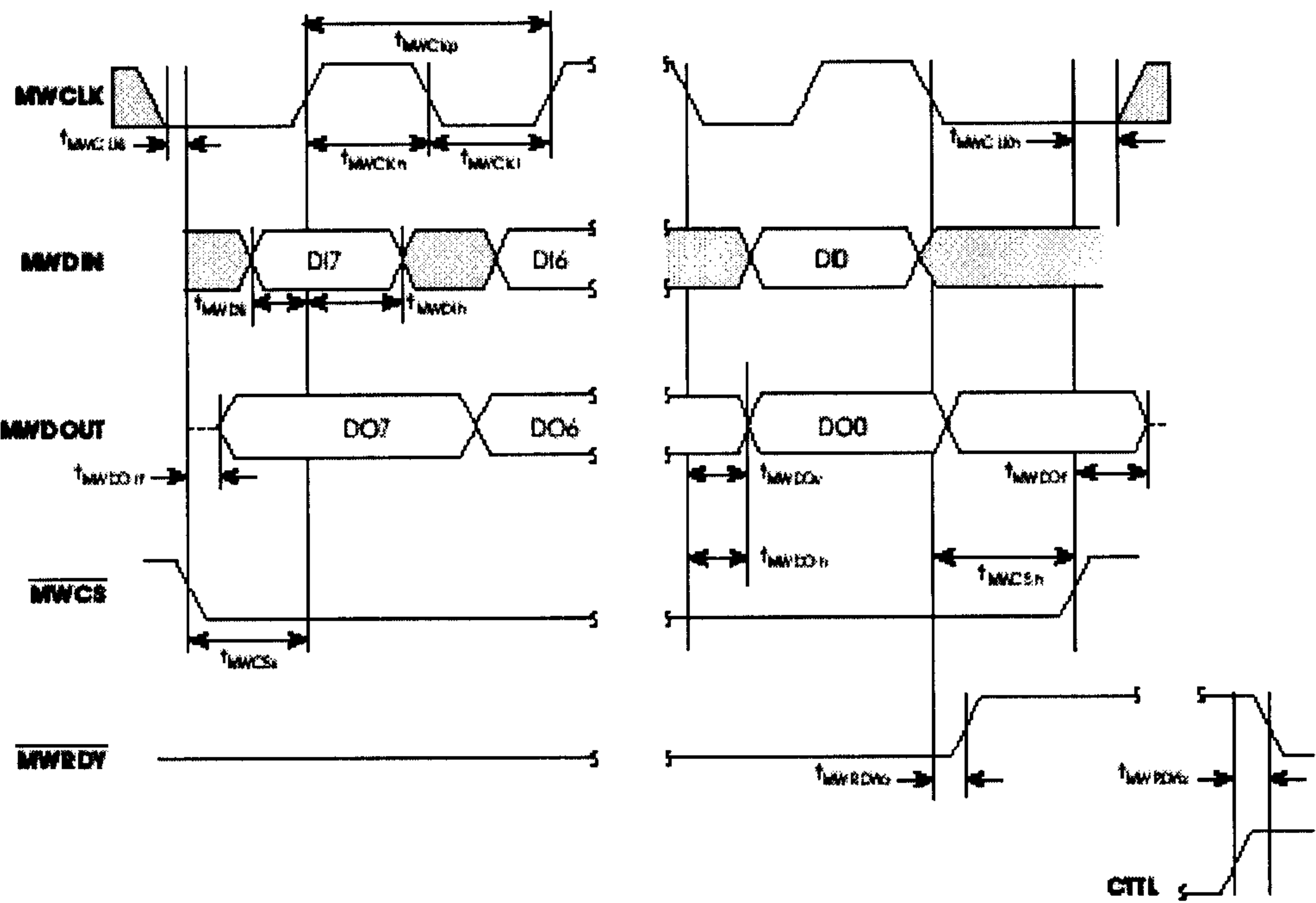
Figure 1-17: MICROWIRE Transaction Timing--Data Transmitted to Output
