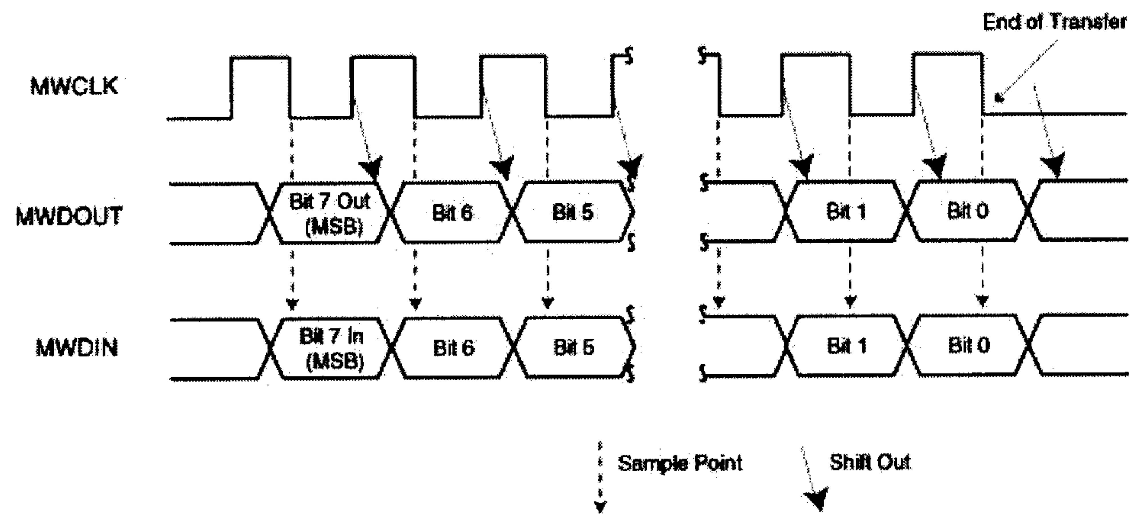
Figure 2-4: Master MircroWIRE Data Transfer
