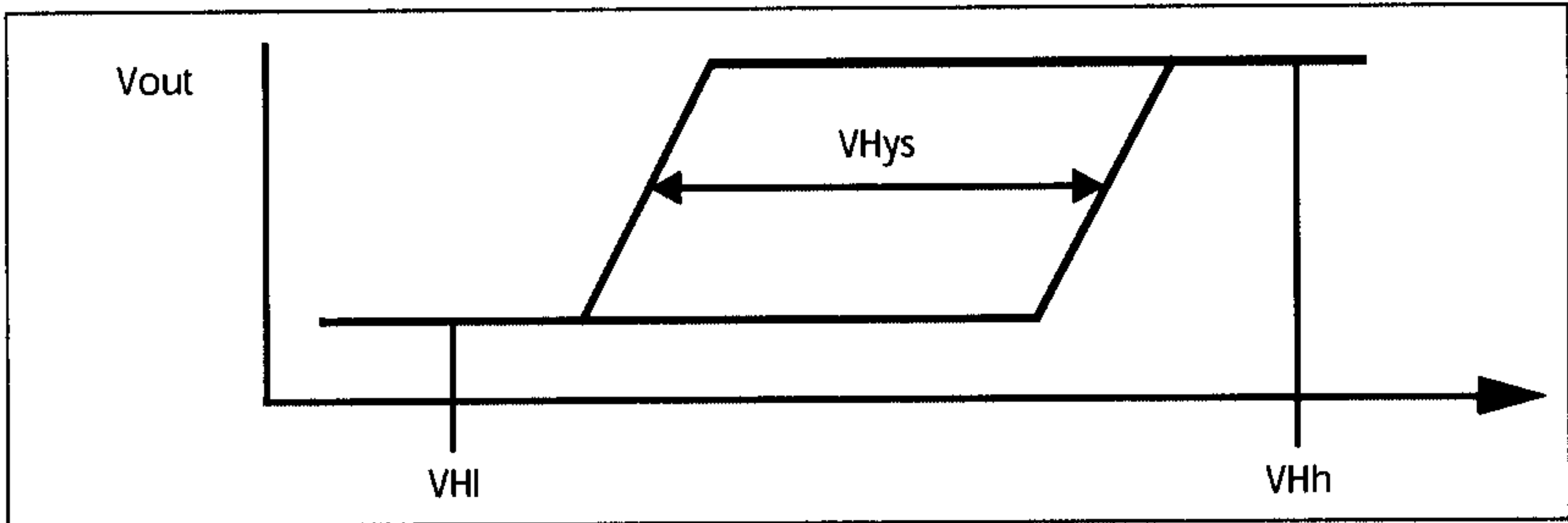
Figure 1-12: Hysteresis Input Characteristics
