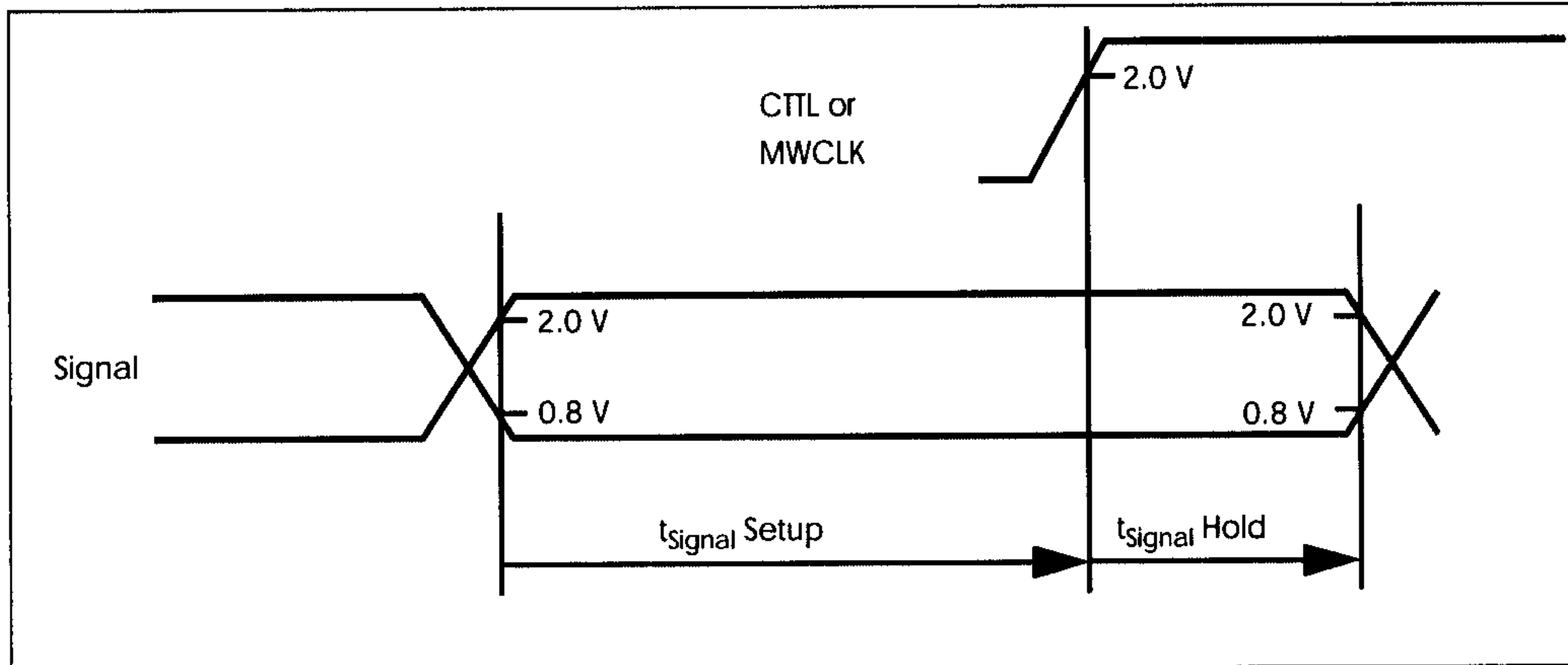
Figure 1-10: Synchronous Input Signals
