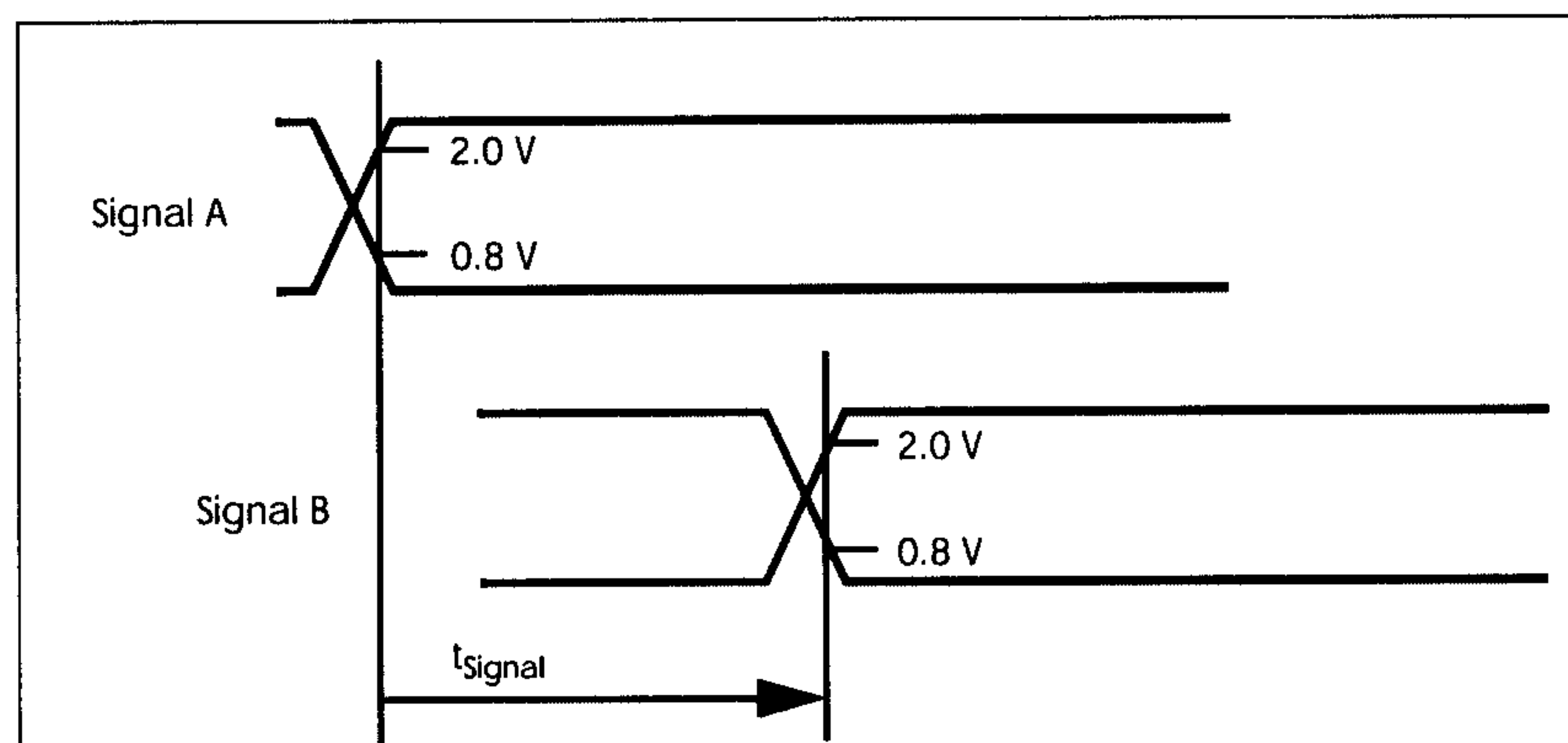
Figure 1-11: Asynchronous Signals
