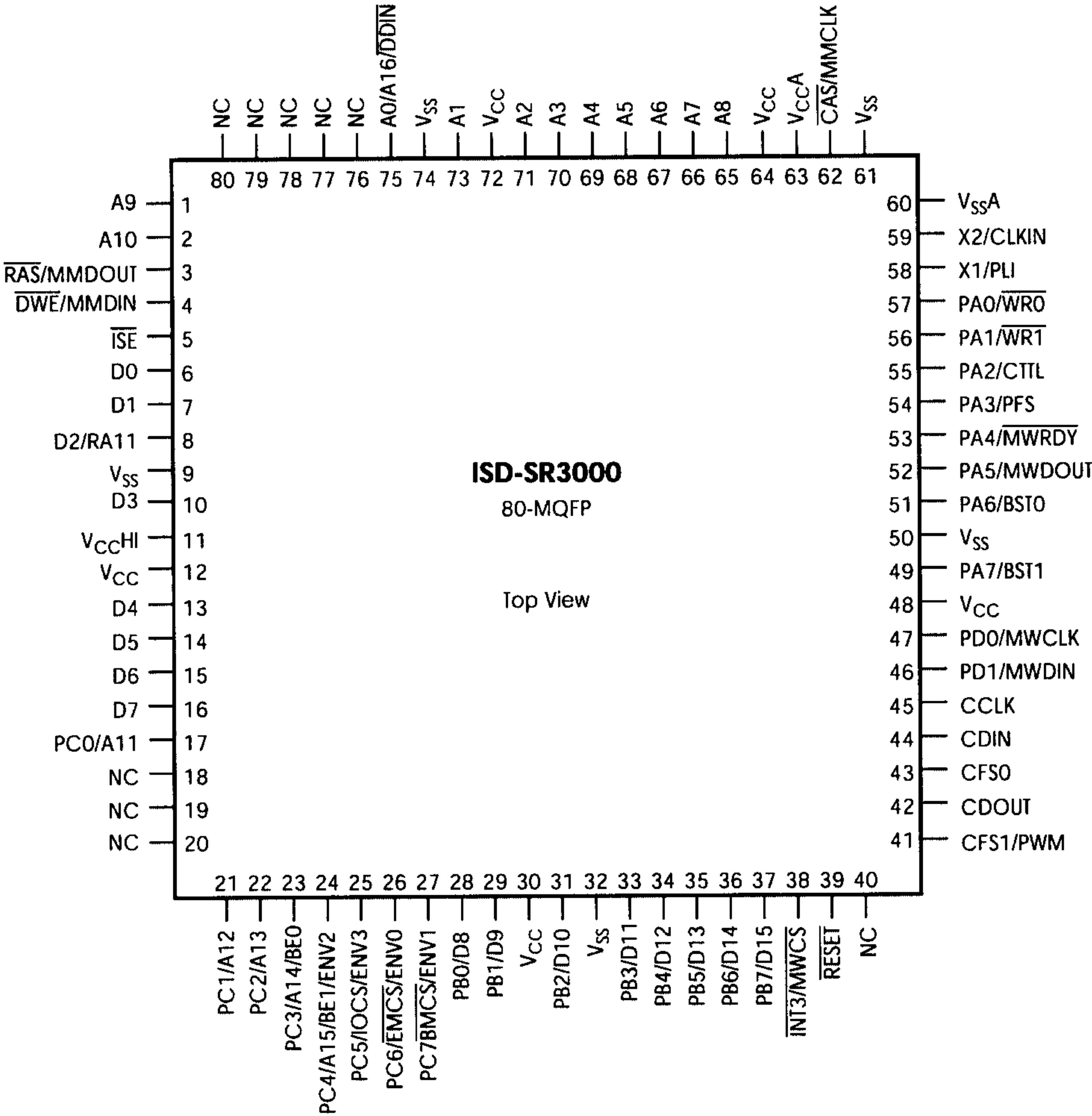
Figure 1-1: 80-MQFP Package Connection Diagram
