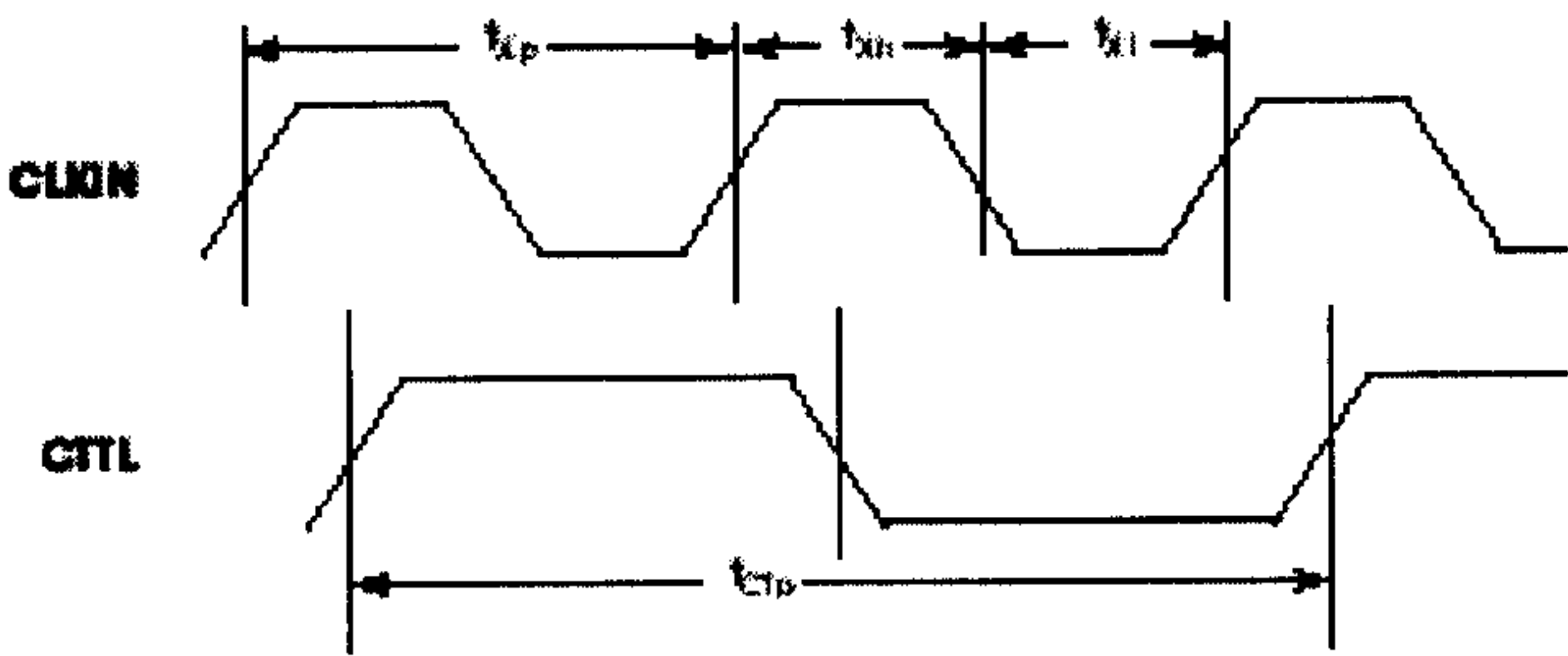
Figure 1-21: CTTL and CLKIN Timing
