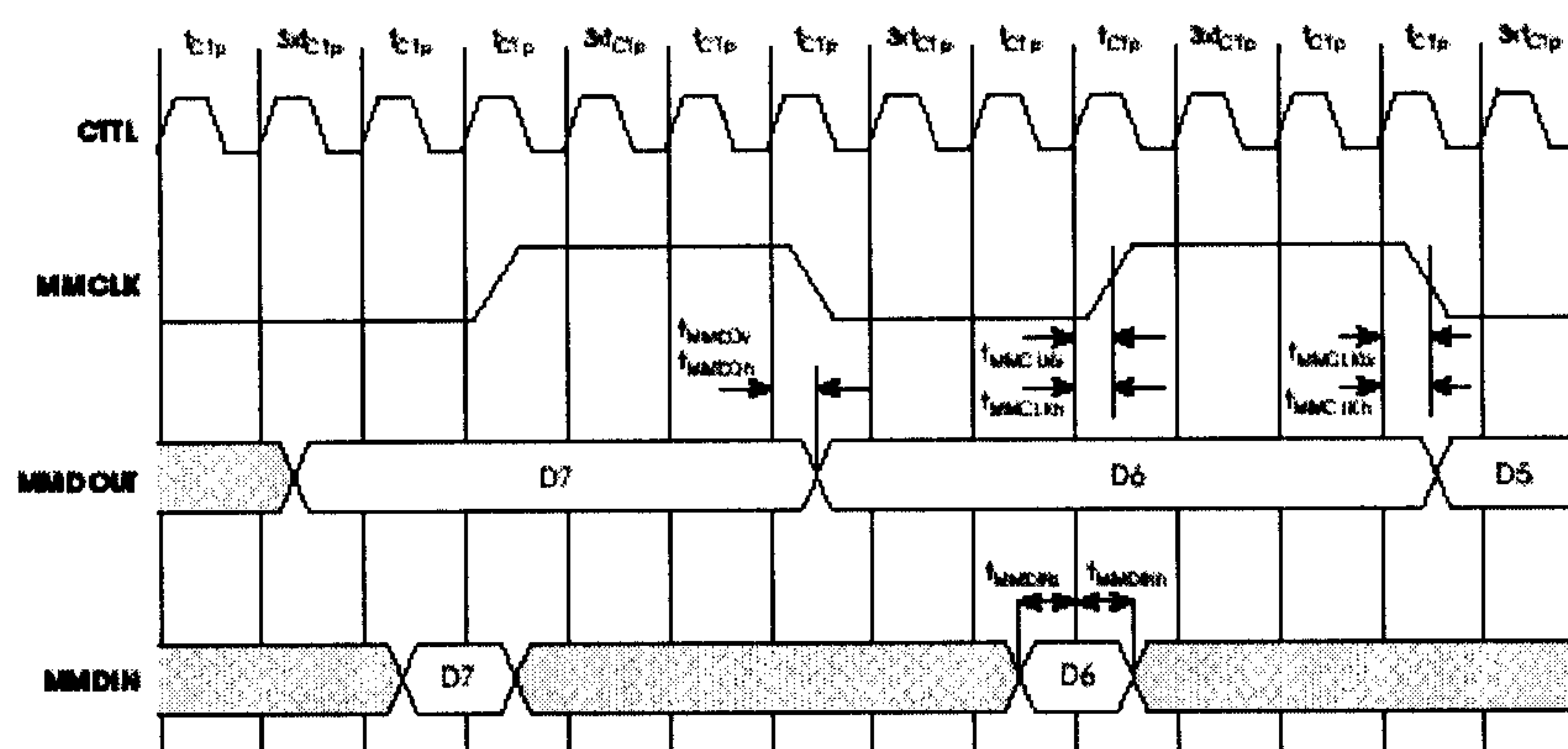
Figure 1-19: Master MICROWIRE Timing
