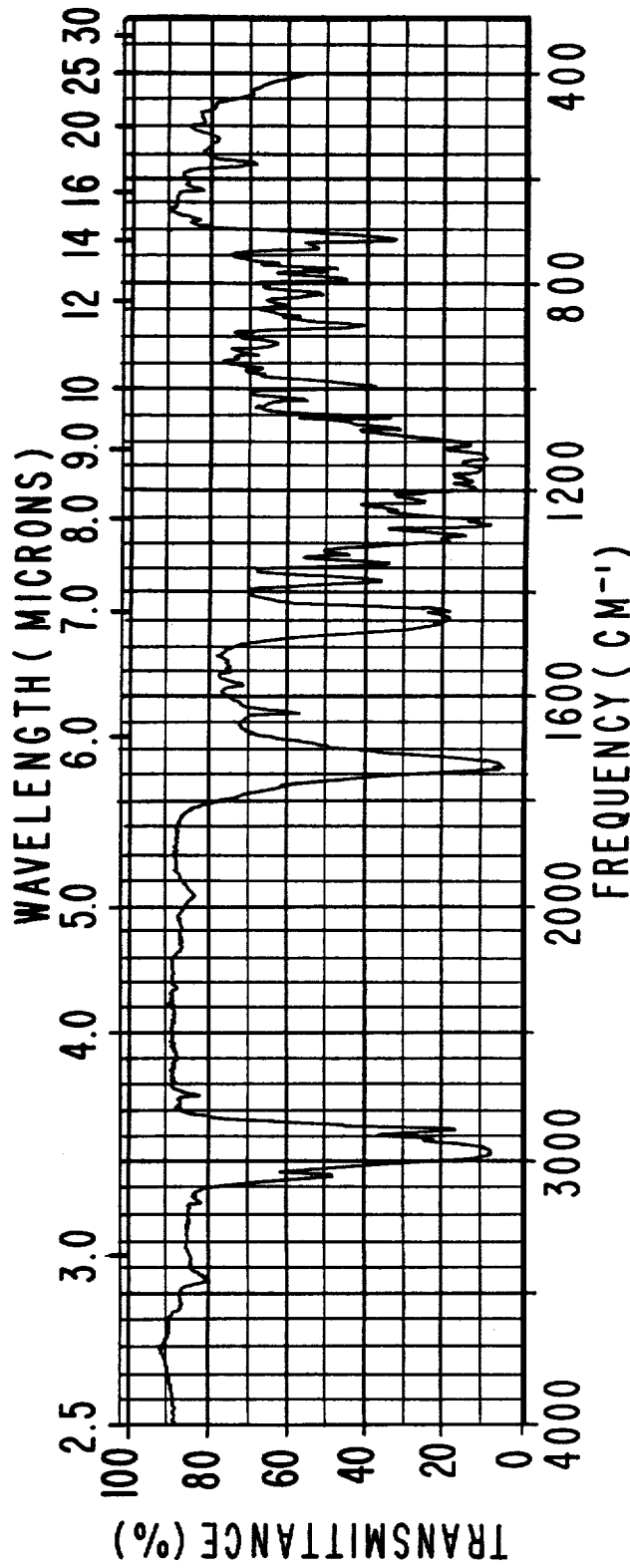
IR SPECTRUM FOR FRACTION 5 OF EXAMPLE I.
