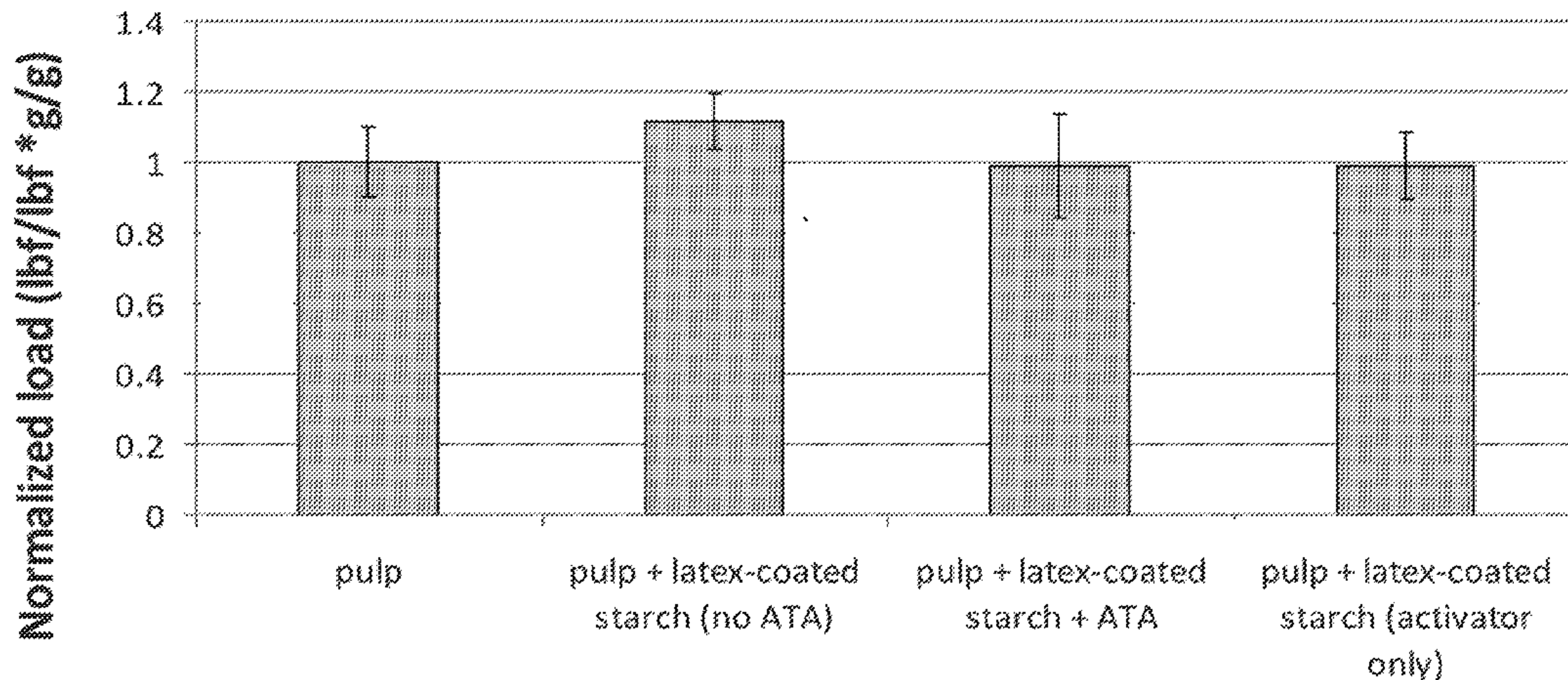
Graph 1: Tensile Strength (Normalized Max. Load)
